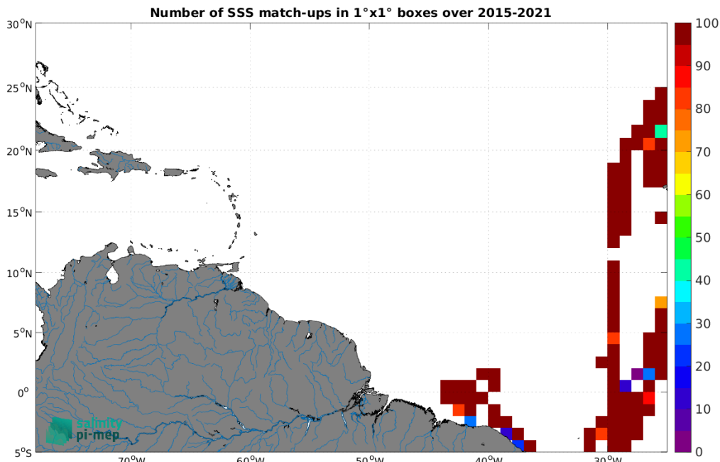
Figure 5: Number of SSS match-ups between TSG (CSIC-UTM) SSS and the SMAP SSS L2 v6 - 40 km (RSS) SSS product for the Amazon and Orinoco river plumes Pi-MEP region over 1^\circ \times 1^\circ boxes and for the full satellite product period.
