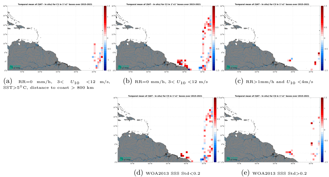
Figure 14: Temporal mean gridded over spatial boxes of size 1^\circ \times 1^\circ of \Delta\text{SSS} (SMAP SSS L2 v6 - 40 km (RSS) - TSG (CSIC-UTM)) for 5 different subdatasets corresponding to:RR=0 mm/h, 3 < U_{10} < 12 m/s, SST >5^\circ\text{C} , distance to coast > 800 km (a), RR=0 mm/h, 3 < U_{10} < 12 m/s (b), RR >1 mm/h and U_{10} < 4 m/s (c), WOA2013 SSS Std <0.2 (d), WOA2013 SSS Std >0.2 (e).
