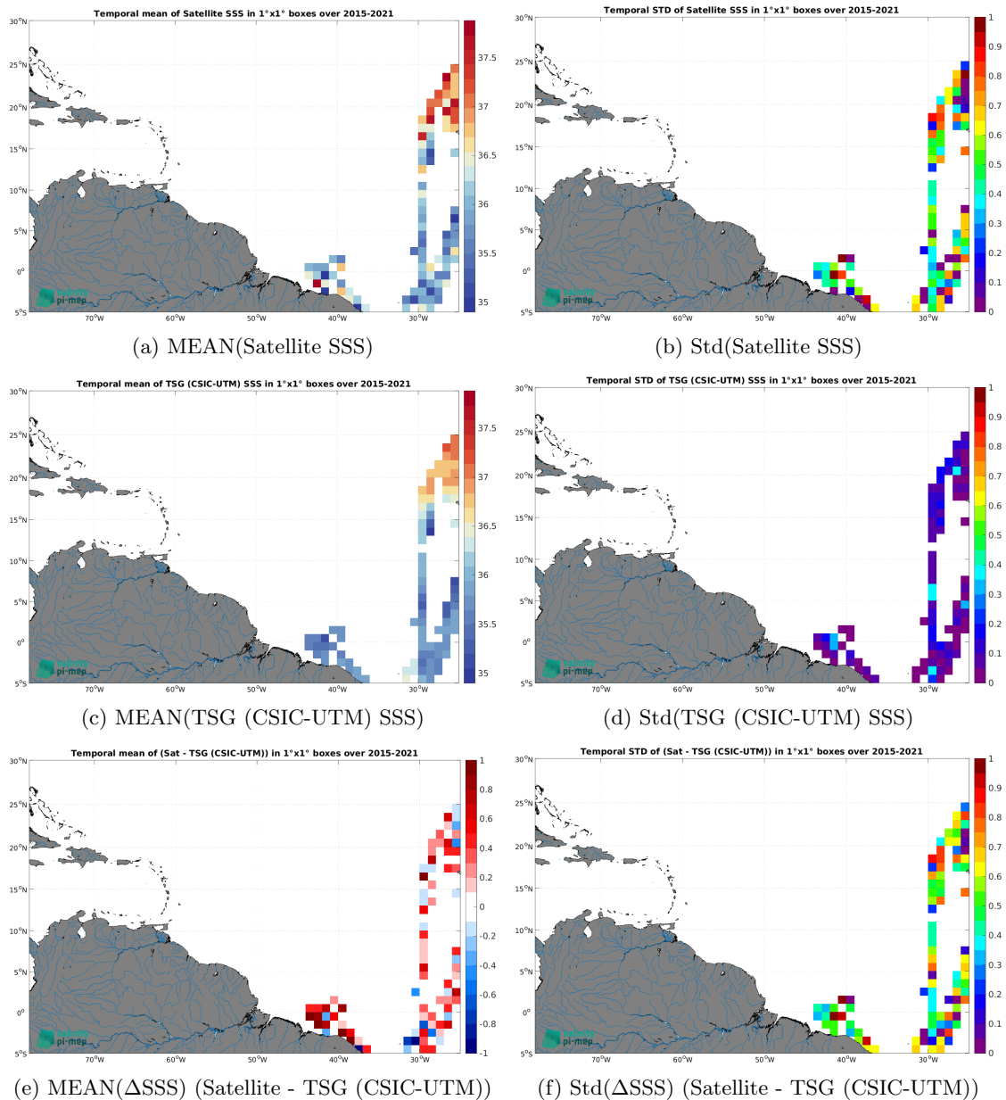
Figure 7: Temporal mean (left) and Std (right) of SSS from SMAP SSS L2 v6 - 40 km (RSS) (top), TSG (CSIC-UTM) (middle), and of \Delta SSS (Satellite - TSG (CSIC-UTM)). Only match-up pairs are used to generate these maps.
