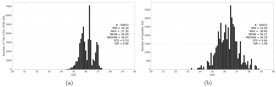
Figure 3: Histograms of SSS from TSG (CSIC-UTM) (a) and SMAP SSS L2 v6 - 40 km (RSS) (b) considering all match-up pairs per bins of 0.1 over the Amazon and Orinoco river plumes Pi-MEP region and for the full satellite product period.
