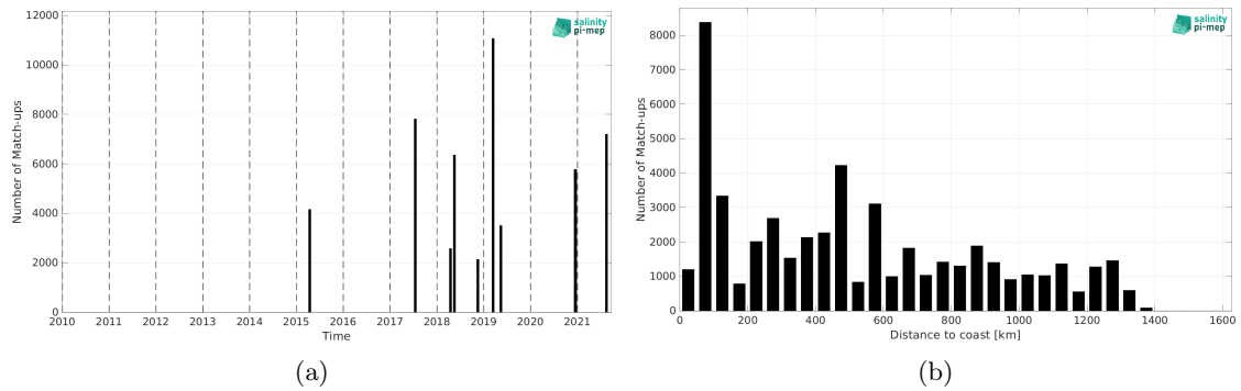
Figure 2: Number of match-ups between TSG (CSIC-UTM) and SMAP SSS L2 v6 - 40 km (RSS) SSS as a function of time (a) and as function of the distance to coast (b) over the Amazon and Orinoco river plumes Pi-MEP region and for the full satellite product period.
