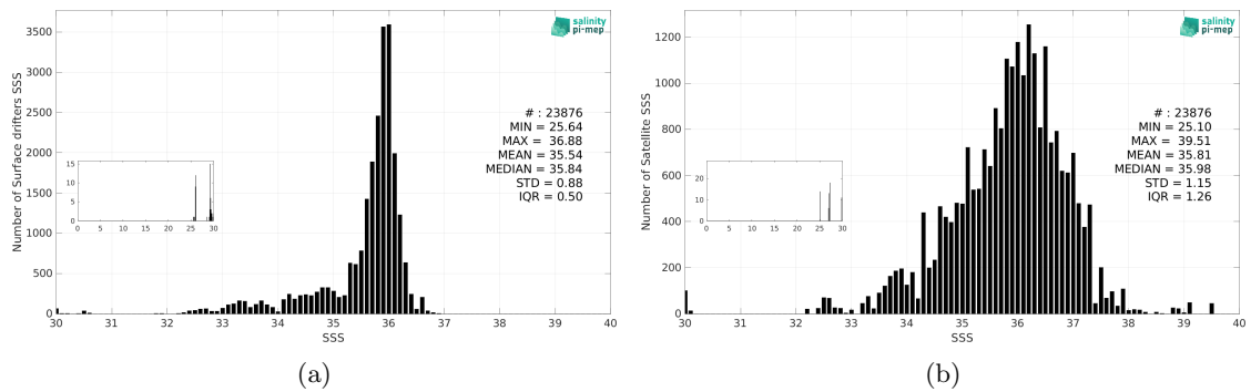
Figure 3: Histograms of SSS from Surface drifters (a) and SMAP SSS L2 v6 - 40 km (RSS) (b) considering all match-up pairs per bins of 0.1 over the Amazon and Orinoco river plumes Pi-MEP region and for the full satellite product period.
