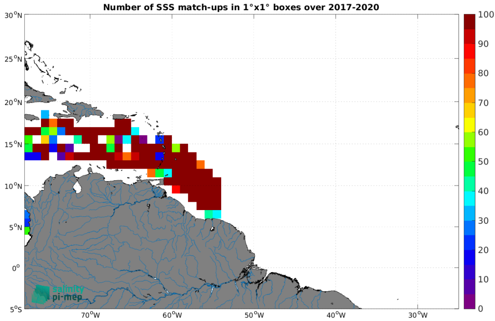
Figure 4: Number of SSS match-ups between Surface drifters SSS and the SMAP SSS L2 v6 - 40 km (RSS) SSS product for the Amazon and Orinoco river plumes Pi-MEP region over 1^\circ \times 1^\circ boxes and for the full satellite product period.
