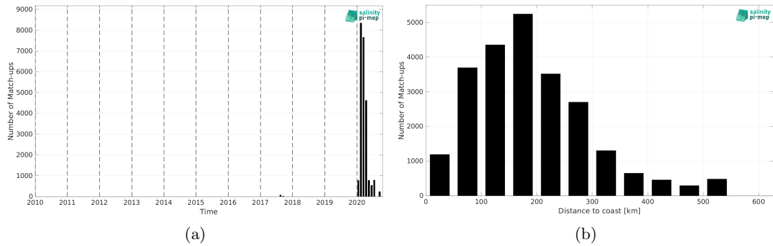
Figure 2: Number of match-ups between Surface drifters and SMAP SSS L2 v6 - 40 km (RSS) SSS as a function of time (a) and as function of the distance to coast (b) over the Amazon and Orinoco river plumes Pi-MEP region and for the full satellite product period.
