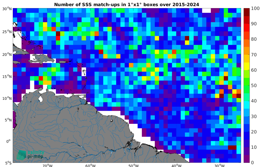
Figure 5: Number of SSS match-ups between Argo SSS and the SMAP SSS L2 v6 - 40 km (RSS) SSS product for the Amazon and Orinoco river plumes Pi-MEP region over 1^\circ \times 1^\circ boxes and for the full satellite product period.
