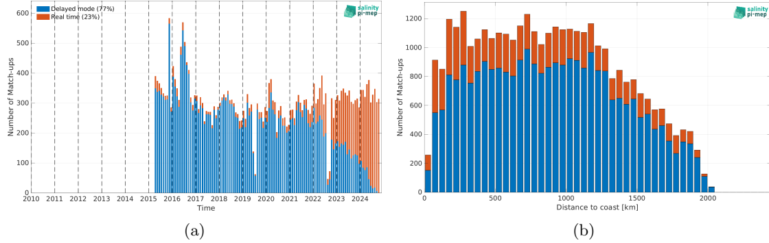
Figure 2: Number of match-ups between Argo and SMAP SSS L2 v6 - 40 km (RSS) SSS as a function of time (a) and as function of the distance to coast (b) over the Amazon and Orinoco river plumes Pi-MEP region and for the full satellite product period.
