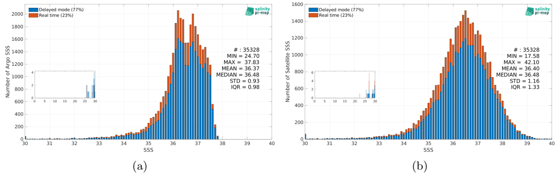
Figure 3: Histograms of SSS from Argo (a) and SMAP SSS L2 v6 - 40 km (RSS) (b) considering all match-up pairs per bins of 0.1 over the Amazon and Orinoco river plumes Pi-MEP region and for the full satellite product period.
