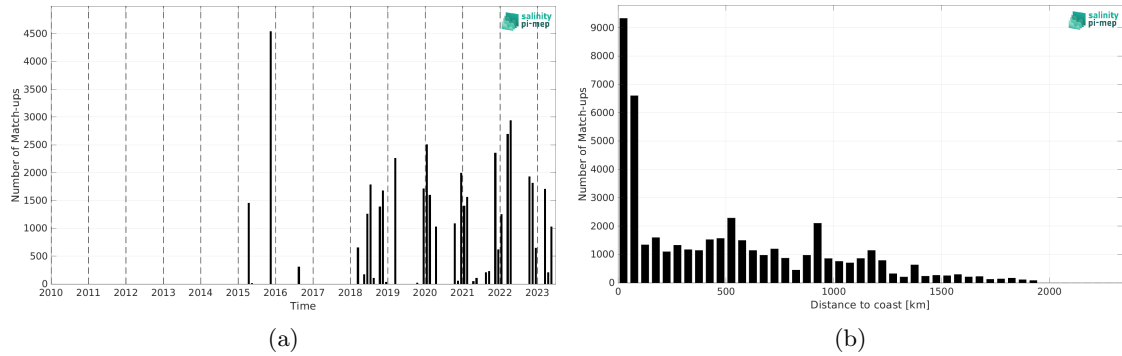
Figure 1: Number of match-ups between TSG (SAMOS) and SMAP SSS L2 v5 (RSS) SSS as a function of time (a) and as function of the distance to coast (b) over the Amazon and Orinoco river plumes Pi-MEP region and for the full satellite product period.
