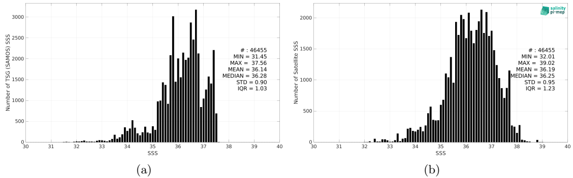
Figure 2: Histograms of SSS from TSG (SAMOS) (a) and SMAP SSS L2 v5 (RSS) (b) considering all match-up pairs per bins of 0.1 over the Amazon and Orinoco river plumes Pi-MEP region and for the full satellite product period.
