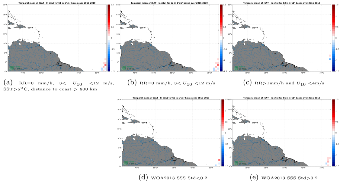
Figure 12: Temporal mean gridded over spatial boxes of size 1^\circ \times 1^\circ of \Delta SSS (SMAP SSS L2 v5 (RSS) - TSG (Polarstern)) for 5 different subdatasets corresponding to:RR=0 mm/h, 3 < U_{10} < 12 m/s, SST >5^\circ\text{C} , distance to coast > 800 km (a), RR=0 mm/h, 3 < U_{10} < 12 m/s (b), RR >1 mm/h and U_{10} < 4 m/s (c), WOA2013 SSS Std <0.2 (d), WOA2013 SSS Std >0.2 (e).
