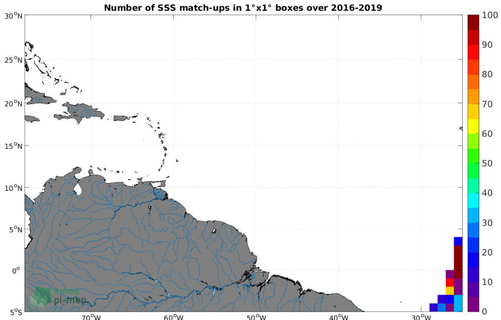
Figure 4: Number of SSS match-ups between TSG (Polarstern) SSS and the SMAP SSS L2 v5 (RSS) SSS product for the Amazon and Orinoco river plumes Pi-MEP region over 1^\circ \times 1^\circ boxes and for the full satellite product period.
