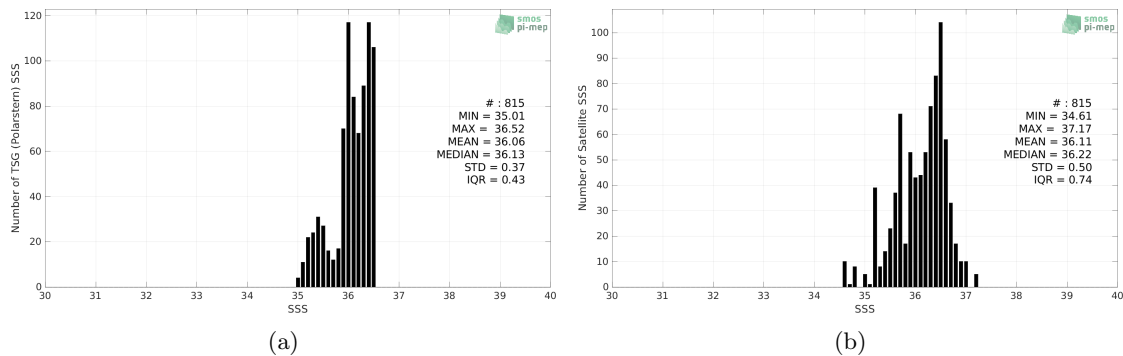
Figure 2: Histograms of SSS from TSG (Polarstern) (a) and SMAP SSS L2 v5 (RSS) (b) considering all match-up pairs per bins of 0.1 over the Amazon and Orinoco river plumes Pi-MEP region and for the full satellite product period.
