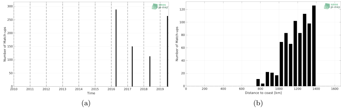
Figure 1: Number of match-ups between TSG (Polarstern) and SMAP SSS L2 v5 (RSS) SSS as a function of time (a) and as function of the distance to coast (b) over the Amazon and Orinoco river plumes Pi-MEP region and for the full satellite product period.
