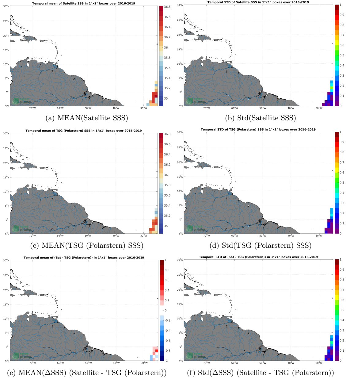
Figure 6: Temporal mean (left) and Std (right) of SSS from SMAP SSS L2 v5 (RSS) (top), TSG (Polarstern) (middle), and of \Delta SSS (Satellite - TSG (Polarstern)). Only match-up pairs are used to generate these maps.
