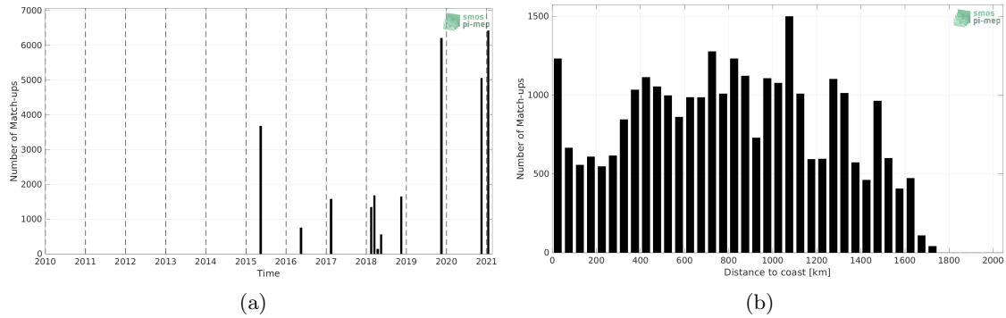
Figure 1: Number of match-ups between TSG (GOSUD-Sailing-ship) and SMAP SSS L2 v5 (RSS) SSS as a function of time (a) and as function of the distance to coast (b) over the Amazon and Orinoco river plumes Pi-MEP region and for the full satellite product period.
