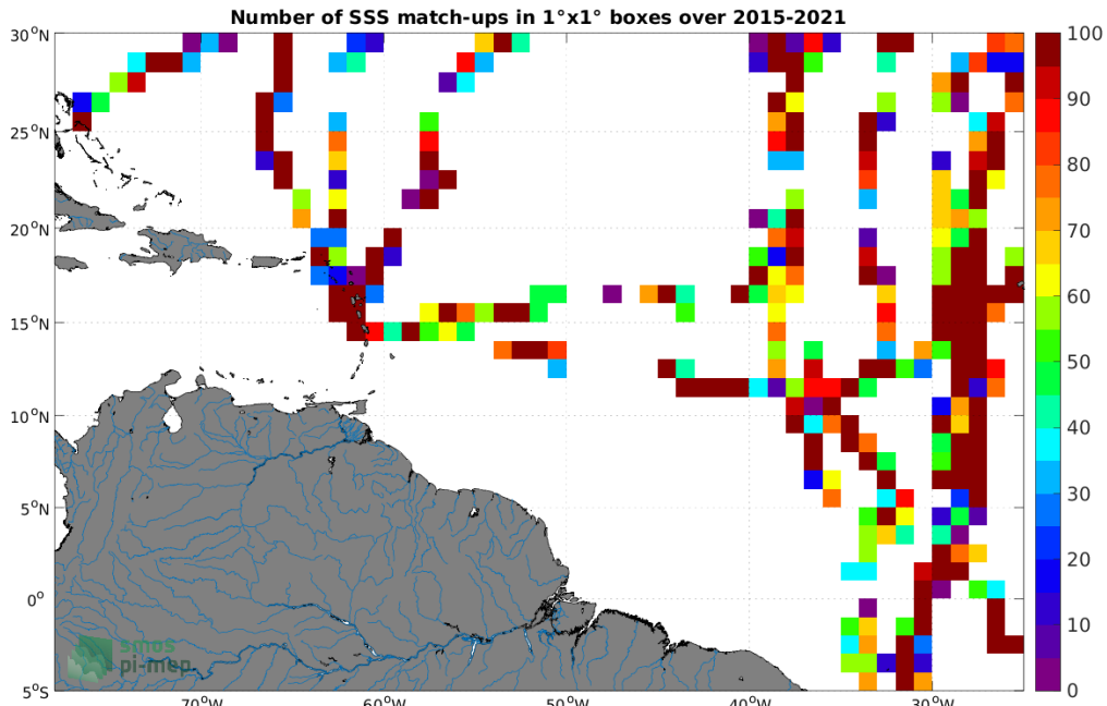
Figure 4: Number of SSS match-ups between TSG (GOSUD-Sailing-ship) SSS and the SMAP SSS L2 v5 (RSS) SSS product for the Amazon and Orinoco river plumes Pi-MEP region over 1^\circ \times 1^\circ boxes and for the full satellite product period.
