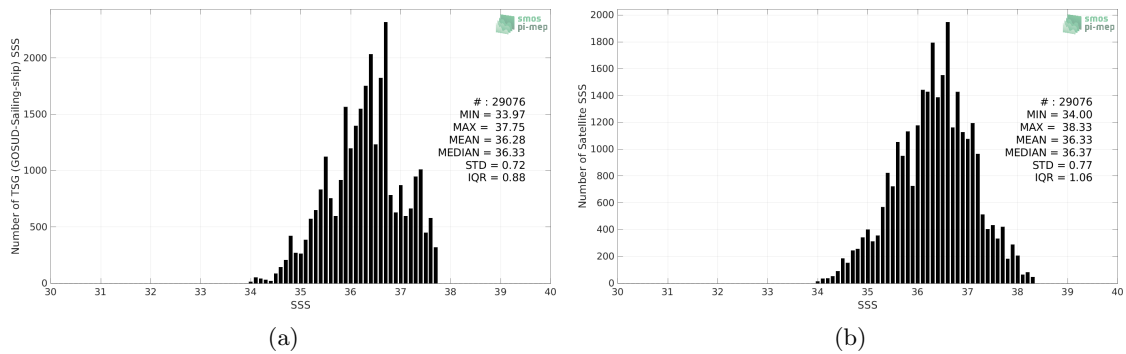
Figure 2: Histograms of SSS from TSG (GOSUD-Sailing-ship) (a) and SMAP SSS L2 v5 (RSS) (b) considering all match-up pairs per bins of 0.1 over the Amazon and Orinoco river plumes Pi-MEP region and for the full satellite product period.
