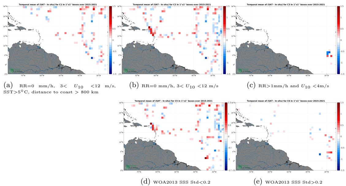
Figure 12: Temporal mean gridded over spatial boxes of size 1^\circ \times 1^\circ of \Delta SSS (SMAP SSS L2 v5 (RSS) - TSG (GOSUD-Sailing-ship)) for 5 different subdatasets corresponding to: RR=0 mm/h, 3 < U_{10} < 12 m/s, SST > 5°C, distance to coast > 800 km (a), RR=0 mm/h, 3 < U_{10} < 12 m/s (b), RR > 1mm/h and U_{10} < 4 m/s (c), WOA2013 SSS Std < 0.2 (d), WOA2013 SSS Std > 0.2 (e).
