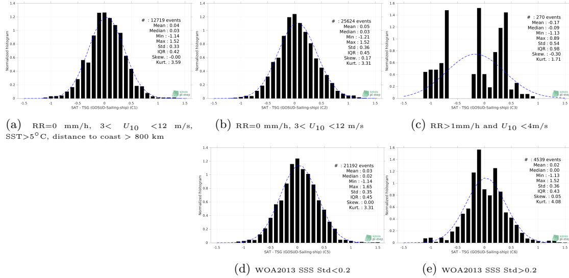
Figure 13: Normalized histogram of \Delta\text{SSS} (SMAP SSS L2 v5 (RSS) - TSG (GOSUD-Sailing-ship)) for 5 different subdatasets corresponding to: RR=0 mm/h, 3 < U_{10} < 12 m/s, SST>5°C, distance to coast > 800 km (a), RR=0 mm/h, 3 < U_{10} < 12 m/s (b), RR>1mm/h and U_{10} < 4 m/s (c), WOA2013 SSS Std<0.2 (d), WOA2013 SSS Std>0.2 (e).
