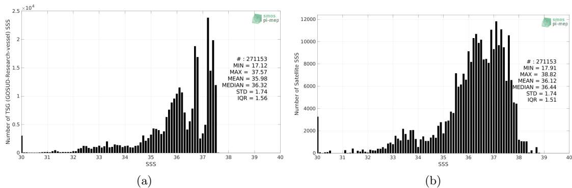
Figure 2: Histograms of SSS from TSG (GOSUD-Research-vessel) (a) and SMAP SSS L2 v5 (RSS) (b) considering all match-up pairs per bins of 0.1 over the Amazon and Orinoco river plumes Pi-MEP region and for the full satellite product period.
