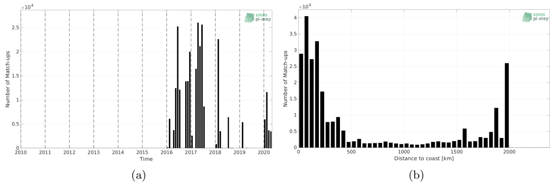
Figure 1: Number of match-ups between TSG (GOSUD-Research-vessel) and SMAP SSS L2 v5 (RSS) SSS as a function of time (a) and as function of the distance to coast (b) over the Amazon and Orinoco river plumes Pi-MEP region and for the full satellite product period.
