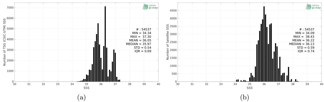
Figure 2: Histograms of SSS from TSG (CSIC-UTM) (a) and SMAP SSS L2 v5 (RSS) (b) considering all match-up pairs per bins of 0.1 over the Amazon and Orinoco river plumes Pi-MEP region and for the full satellite product period.
