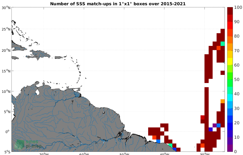
Figure 4: Number of SSS match-ups between TSG (CSIC-UTM) SSS and the SMAP SSS L2 v5 (RSS) SSS product for the Amazon and Orinoco river plumes Pi-MEP region over 1^\circ \times 1^\circ boxes and for the full satellite product period.
