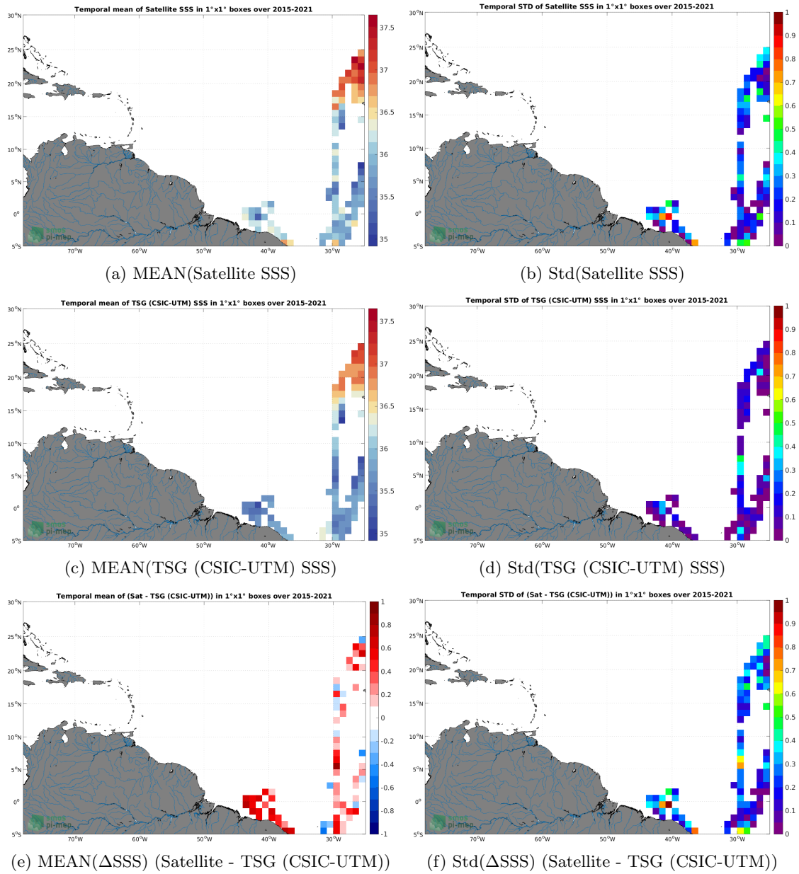
Figure 6: Temporal mean (left) and Std (right) of SSS from SMAP SSS L2 v5 (RSS) (top), TSG (CSIC-UTM) (middle), and of \Delta SSS (Satellite - TSG (CSIC-UTM)). Only match-up pairs are used to generate these maps.
