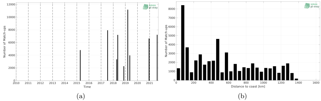
Figure 1: Number of match-ups between TSG (CSIC-UTM) and SMAP SSS L2 v5 (RSS) SSS as a function of time (a) and as function of the distance to coast (b) over the Amazon and Orinoco river plumes Pi-MEP region and for the full satellite product period.
