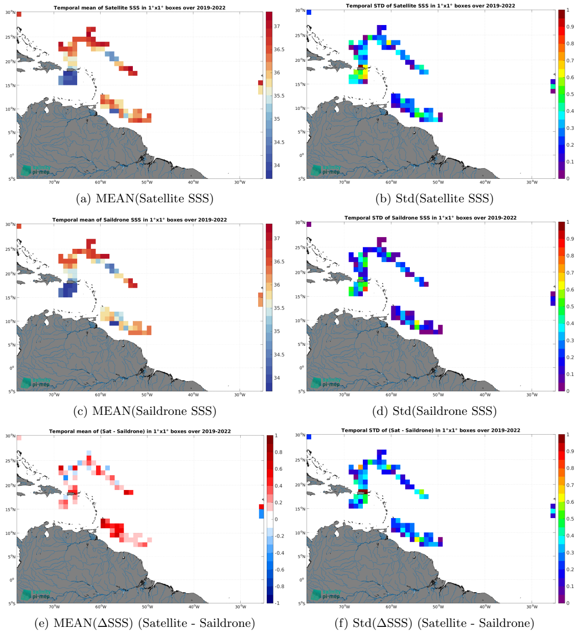
Figure 6: Temporal mean (left) and Std (right) of SSS from SMAP SSS L2 v5 (RSS) (top), Saildrone (middle), and of \Delta SSS (Satellite - Saildrone). Only match-up pairs are used to generate these maps.
