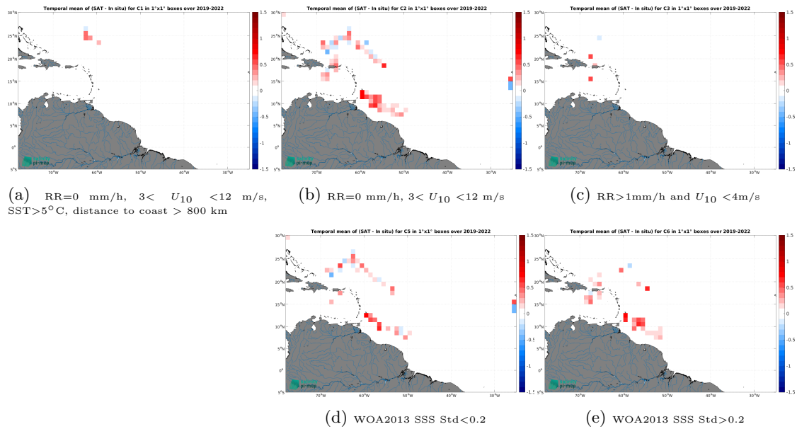
Figure 12: Temporal mean gridded over spatial boxes of size 1^\circ \times 1^\circ of \Delta SSS (SMAP SSS L2 v5 (RSS) - Saldrone) for 5 different subdatasets corresponding to:RR=0 mm/h, 3 < U_{10} < 12 m/s, SST >5^\circ\text{C} , distance to coast > 800 km (a), RR=0 mm/h, 3 < U_{10} < 12 m/s (b), RR >1 mm/h and U_{10} < 4 m/s (c), WOA2013 SSS Std <0.2 (d), WOA2013 SSS Std >0.2 (e).
