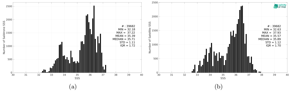
Figure 2: Histograms of SSS from Saildrone (a) and SMAP SSS L2 v5 (RSS) (b) considering all match-up pairs per bins of 0.1 over the Amazon and Orinoco river plumes Pi-MEP region and for the full satellite product period.
