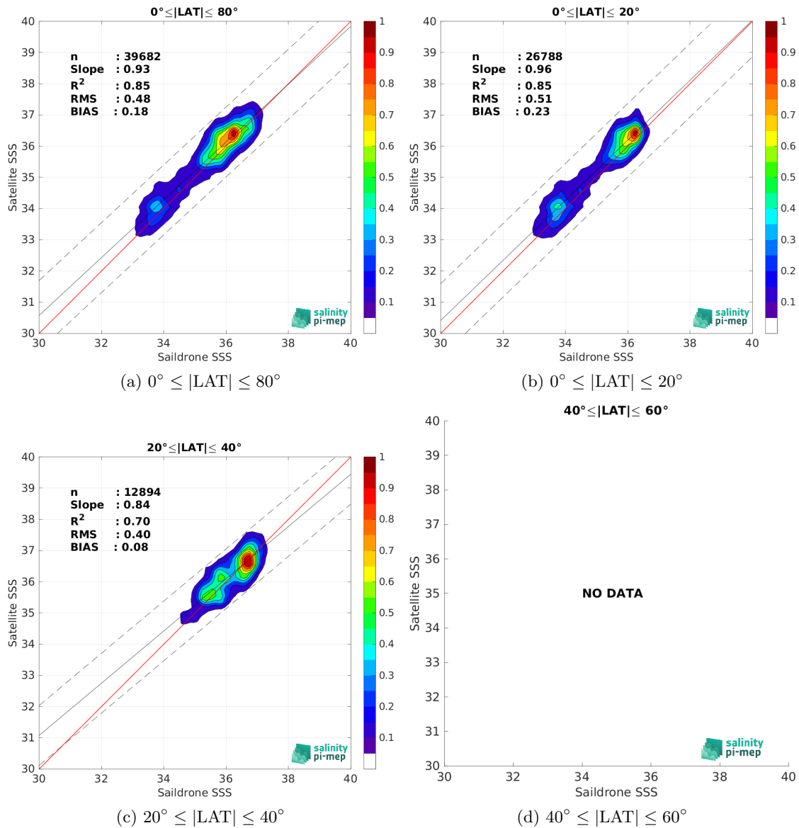
Figure 9: Contour maps of the concentration of SMAP SSS L2 v5 (RSS) SSS (y-axis) versus Sailldrone SSS (x-axis) at match-up pairs for different latitude bands. For each plot, the red line shows x=y . The black thin and dashed lines indicate a linear fit through the data cloud and the \pm 95\% confidence levels, respectively. The number match-up pairs n , the slope and R^2 coefficient of the linear fit, the root mean square (RMS) and the mean bias between satellite and in situ data are indicated for each latitude band in each plots.
