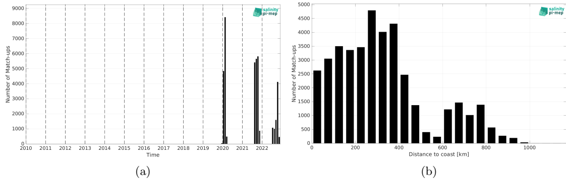
Figure 1: Number of match-ups between Saildrone and SMAP SSS L2 v5 (RSS) SSS as a function of time (a) and as function of the distance to coast (b) over the Amazon and Orinoco river plumes Pi-MEP region and for the full satellite product period.
