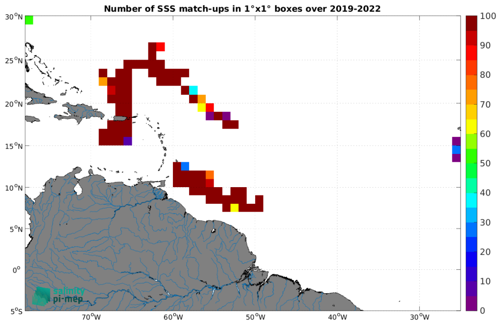
Figure 4: Number of SSS match-ups between Saildrone SSS and the SMAP SSS L2 v5 (RSS) SSS product for the Amazon and Orinoco river plumes Pi-MEP region over 1^\circ \times 1^\circ boxes and for the full satellite product period.
