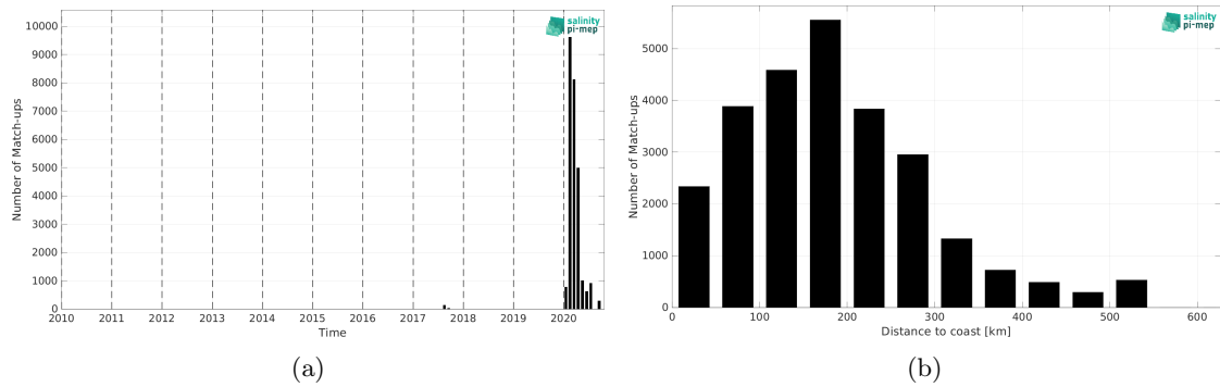
Figure 1: Number of match-ups between Surface drifters and SMAP SSS L2 v5 (RSS) SSS as a function of time (a) and as function of the distance to coast (b) over the Amazon and Orinoco river plumes Pi-MEP region and for the full satellite product period.
