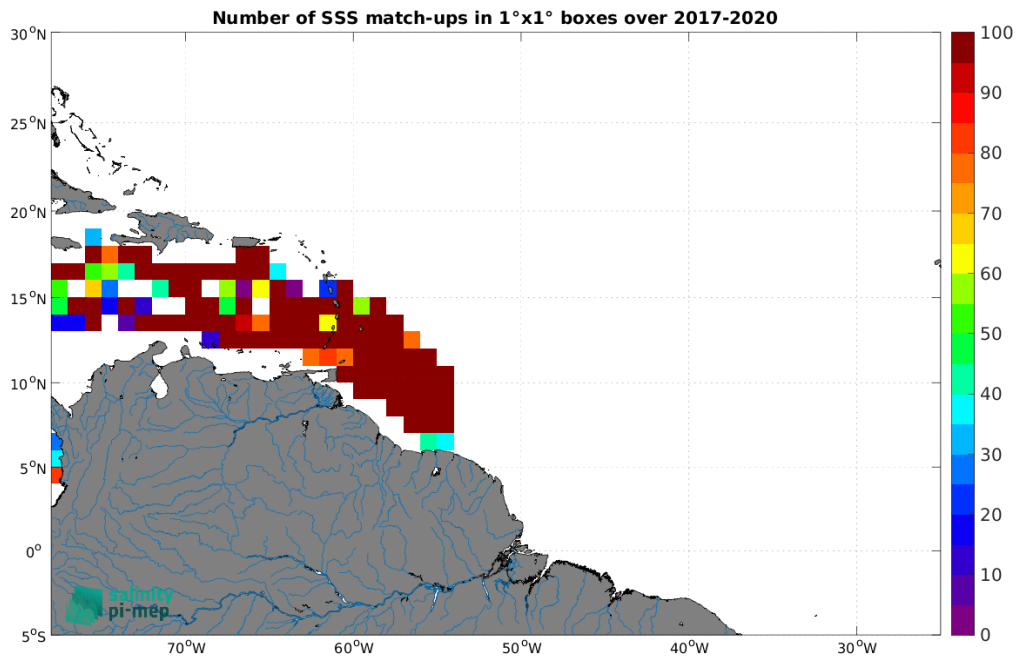
Figure 3: Number of SSS match-ups between Surface drifters SSS and the SMAP SSS L2 v5 (RSS) SSS product for the Amazon and Orinoco river plumes Pi-MEP region over 1°x1° boxes and for the full satellite product period.
