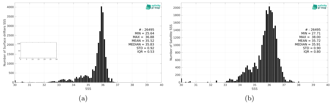
Figure 2: Histograms of SSS from Surface drifters (a) and SMAP SSS L2 v5 (RSS) (b) considering all match-up pairs per bins of 0.1 over the Amazon and Orinoco river plumes Pi-MEP region and for the full satellite product period.
