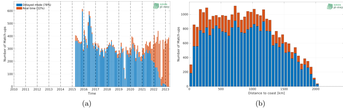
Figure 1: Number of match-ups between Argo and SMAP SSS L2 v5 (RSS) SSS as a function of time (a) and as function of the distance to coast (b) over the Amazon and Orinoco river plumes Pi-MEP region and for the full satellite product period.
