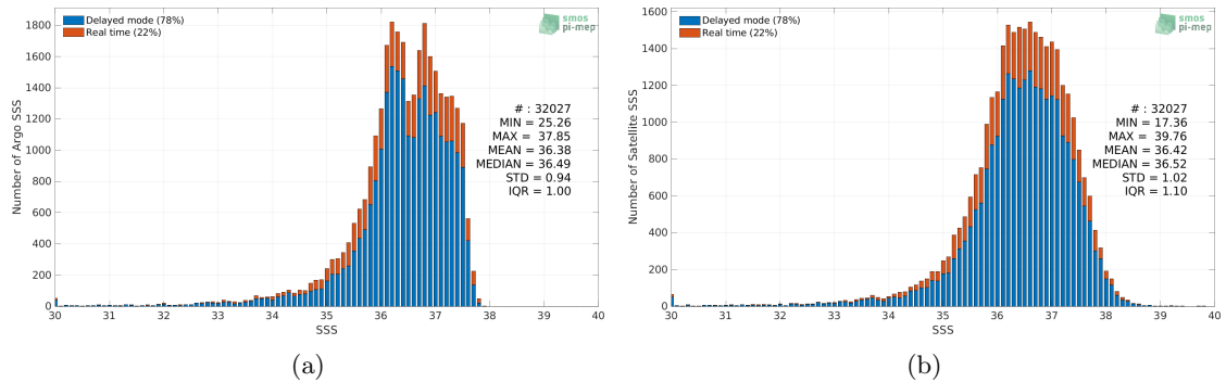
Figure 2: Histograms of SSS from Argo (a) and SMAP SSS L2 v5 (RSS) (b) considering all match-up pairs per bins of 0.1 over the Amazon and Orinoco river plumes Pi-MEP region and for the full satellite product period.
