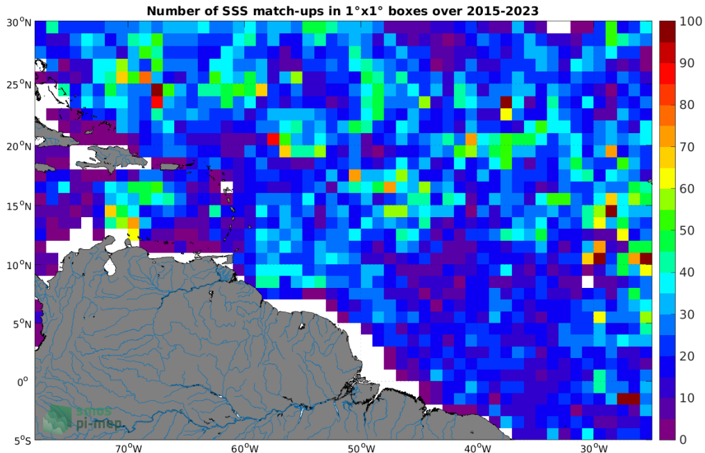
Figure 4: Number of SSS match-ups between Argo SSS and the SMAP SSS L2 v5 (RSS) SSS product for the Amazon and Orinoco river plumes Pi-MEP region over 1^\circ \times 1^\circ boxes and for the full satellite product period.
