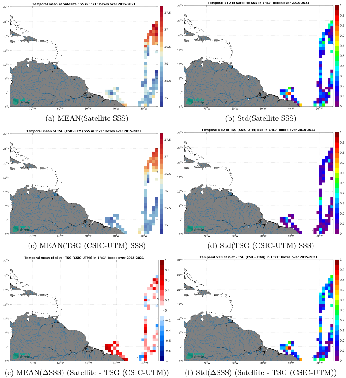
Figure 7: Temporal mean (left) and Std (right) of SSS from SMAP SSS L2 v5.3 (RSS) (top), TSG (CSIC-UTM) (middle), and of \Delta SSS (Satellite - TSG (CSIC-UTM)). Only match-up pairs are used to generate these maps.
