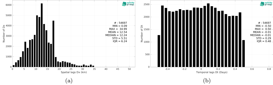
Figure 6: Histograms of the spatial (a) and temporal (b) lags between the location/time of the TSG (CSIC-UTM) measurement and the date of the corresponding SMAP SSS L2 v5.3 (RSS) SSS pixel.
