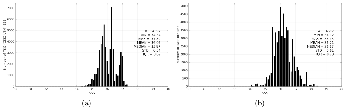
Figure 3: Histograms of SSS from TSG (CSIC-UTM) (a) and SMAP SSS L2 v5.3 (RSS) (b) considering all match-up pairs per bins of 0.1 over the Amazon and Orinoco river plumes Pi-MEP region and for the full satellite product period.
