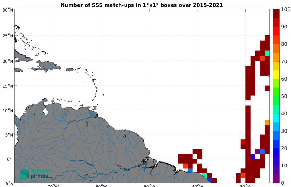
Figure 5: Number of SSS match-ups between TSG (CSIC-UTM) SSS and the SMAP SSS L2 v5.3 (RSS) SSS product for the Amazon and Orinoco river plumes Pi-MEP region over 1^\circ \times 1^\circ boxes and for the full satellite product period.
