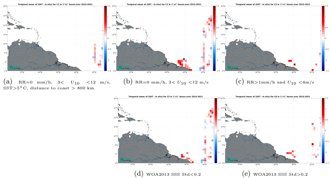
Figure 14: Temporal mean gridded over spatial boxes of size 1^\circ \times 1^\circ of \Delta SSS (SMAP SSS L2 v5.3 (RSS) - TSG (CSIC-UTM)) for 5 different subdatasets corresponding to:RR=0 mm/h, 3 < U_{10} < 12 m/s, SST >5^\circ\text{C} , distance to coast > 800 km (a), RR=0 mm/h, 3 < U_{10} < 12 m/s (b), RR >1 mm/h and U_{10} < 4 m/s (c), WOA2013 SSS Std <0.2 (d), WOA2013 SSS Std >0.2 (e).
