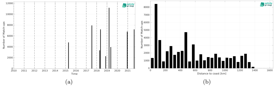
Figure 2: Number of match-ups between TSG (CSIC-UTM) and SMAP SSS L2 v5.3 (RSS) SSS as a function of time (a) and as function of the distance to coast (b) over the Amazon and Orinoco river plumes Pi-MEP region and for the full satellite product period.
