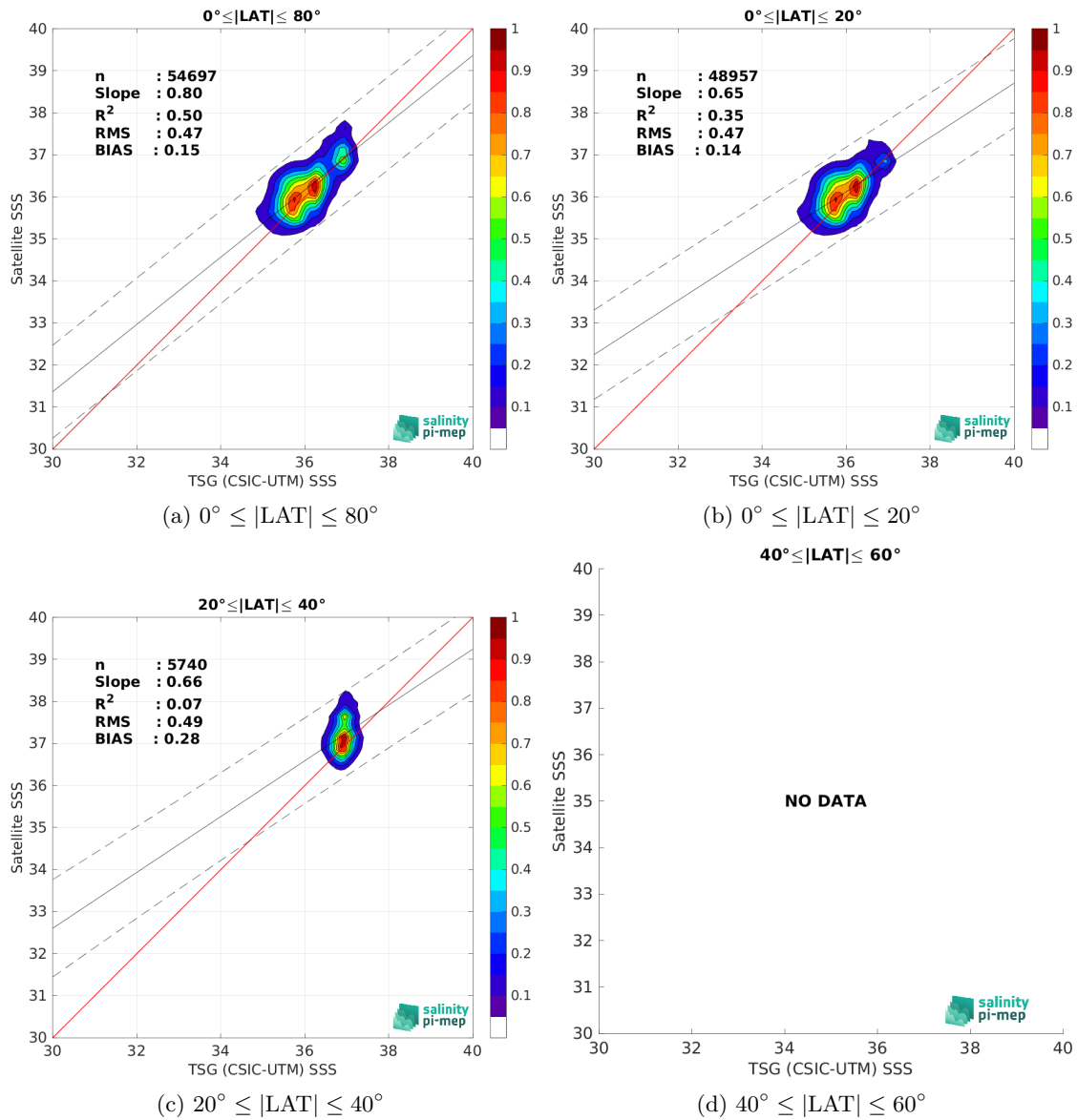
Figure 10: Contour maps of the concentration of SMAP SSS L2 v5.3 (RSS) SSS (y-axis) versus TSG (CSIC-UTM) SSS (x-axis) at match-up pairs for different latitude bands. For each plot, the red line shows x=y . The black thin and dashed lines indicate a linear fit through the data cloud and the \pm 95\% confidence levels, respectively. The number match-up pairs n , the slope and R^2 coefficient of the linear fit, the root mean square (RMS) and the mean bias between satellite and in situ data are indicated for each latitude band in each plots.
