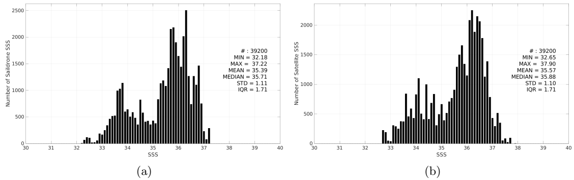
Figure 3: Histograms of SSS from Saildrone (a) and SMAP SSS L2 v5.3 (RSS) (b) considering all match-up pairs per bins of 0.1 over the Amazon and Orinoco river plumes Pi-MEP region and for the full satellite product period.
