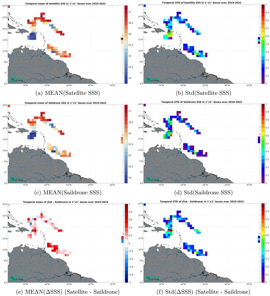
Figure 7: Temporal mean (left) and Std (right) of SSS from SMAP SSS L2 v5.3 (RSS) (top), Saildrone (middle), and of \Delta SSS (Satellite - Saildrone). Only match-up pairs are used to generate these maps.
