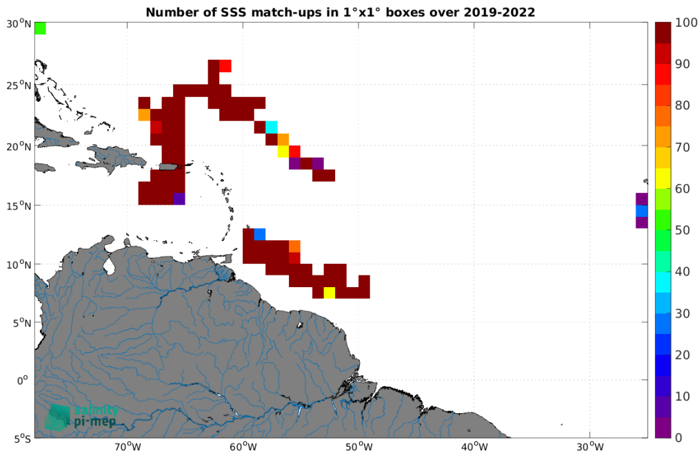
Figure 5: Number of SSS match-ups between Saildrone SSS and the SMAP SSS L2 v5.3 (RSS) SSS product for the Amazon and Orinoco river plumes Pi-MEP region over 1^\circ \times 1^\circ boxes and for the full satellite product period.
