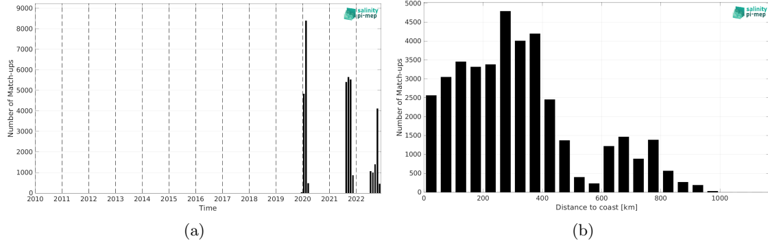
Figure 2: Number of match-ups between Saildrone and SMAP SSS L2 v5.3 (RSS) SSS as a function of time (a) and as function of the distance to coast (b) over the Amazon and Orinoco river plumes Pi-MEP region and for the full satellite product period.
