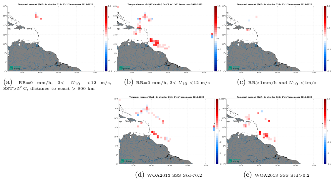
Figure 14: Temporal mean gridded over spatial boxes of size 1^\circ \times 1^\circ of \Delta SSS (SMAP SSS L2 v5.3 (RSS) - Saldrone) for 5 different subdatasets corresponding to:RR=0 mm/h, 3 < U_{10} < 12 m/s, SST>5°C, distance to coast > 800 km (a), RR=0 mm/h, 3 < U_{10} < 12 m/s (b), RR>1mm/h and U_{10} < 4 m/s (c), WOA2013 SSS Std<0.2 (d), WOA2013 SSS Std>0.2 (e).
