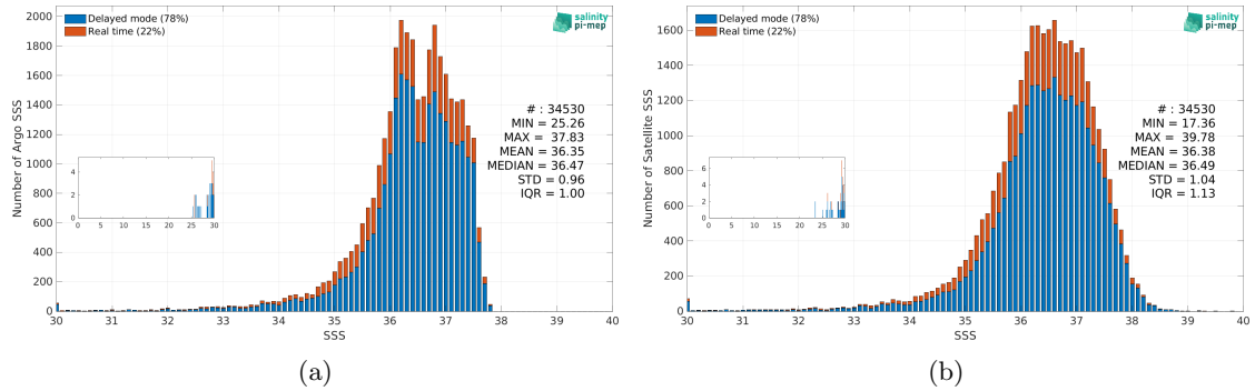
Figure 3: Histograms of SSS from Argo (a) and SMAP SSS L2 v5.3 (RSS) (b) considering all match-up pairs per bins of 0.1 over the Amazon and Orinoco river plumes Pi-MEP region and for the full satellite product period.
