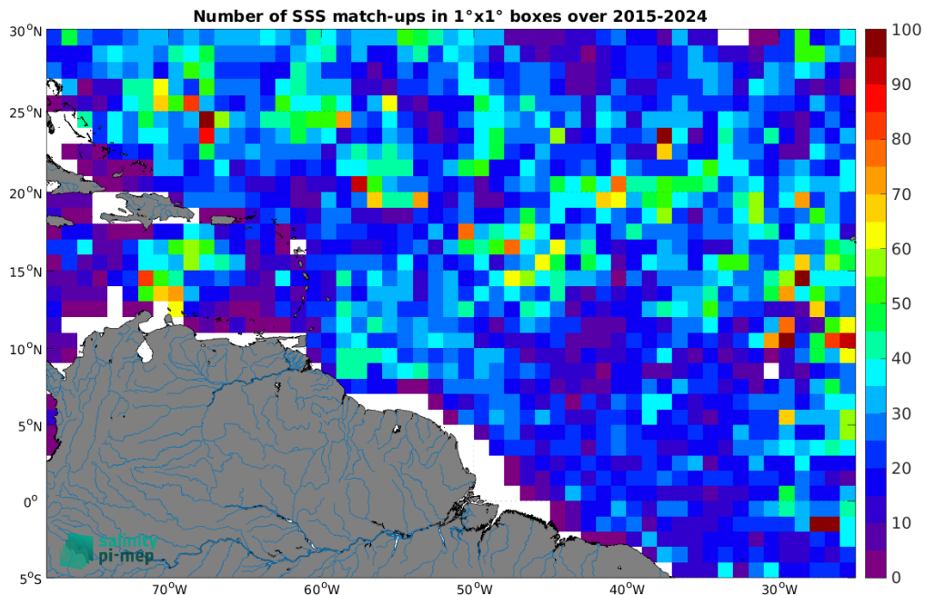
Figure 5: Number of SSS match-ups between Argo SSS and the SMAP SSS L2 v5.3 (RSS) SSS product for the Amazon and Orinoco river plumes Pi-MEP region over 1^\circ \times 1^\circ boxes and for the full satellite product period.
