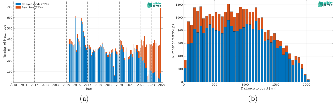
Figure 2: Number of match-ups between Argo and SMAP SSS L2 v5.3 (RSS) SSS as a function of time (a) and as function of the distance to coast (b) over the Amazon and Orinoco river plumes Pi-MEP region and for the full satellite product period.
