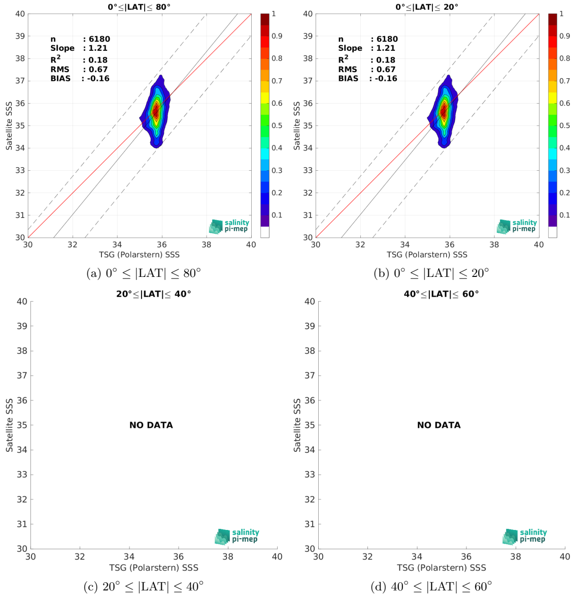
Figure 10: Contour maps of the concentration of SMAP SSS L2 v5.3 - 40 km (RSS) SSS (y-axis) versus TSG (Polarstern) SSS (x-axis) at match-up pairs for different latitude bands. For each plot, the red line shows x=y . The black thin and dashed lines indicate a linear fit through the data cloud and the \pm 95\% confidence levels, respectively. The number match-up pairs n , the slope and R^2 coefficient of the linear fit, the root mean square (RMS) and the mean bias between satellite and in situ data are indicated for each latitude band in each plots.
