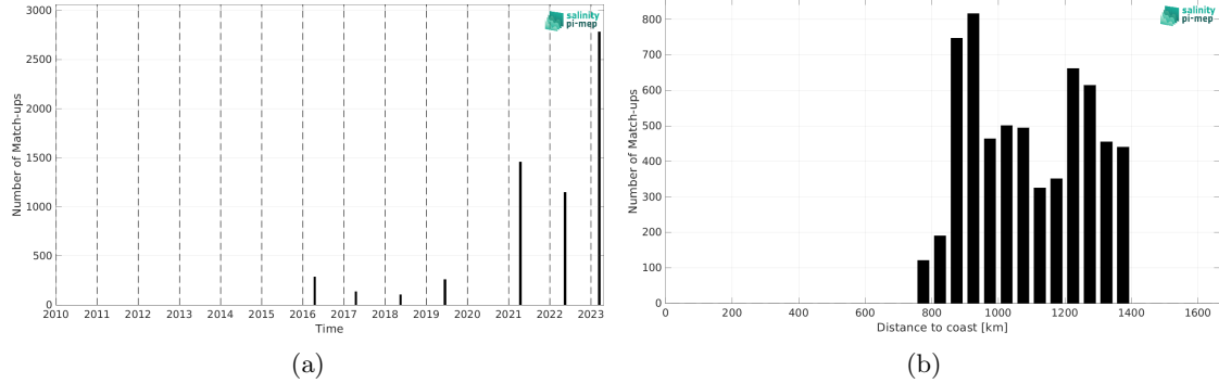
Figure 2: Number of match-ups between TSG (Polarstern) and SMAP SSS L2 v5.3 - 40 km (RSS) SSS as a function of time (a) and as function of the distance to coast (b) over the Amazon and Orinoco river plumes Pi-MEP region and for the full satellite product period.
