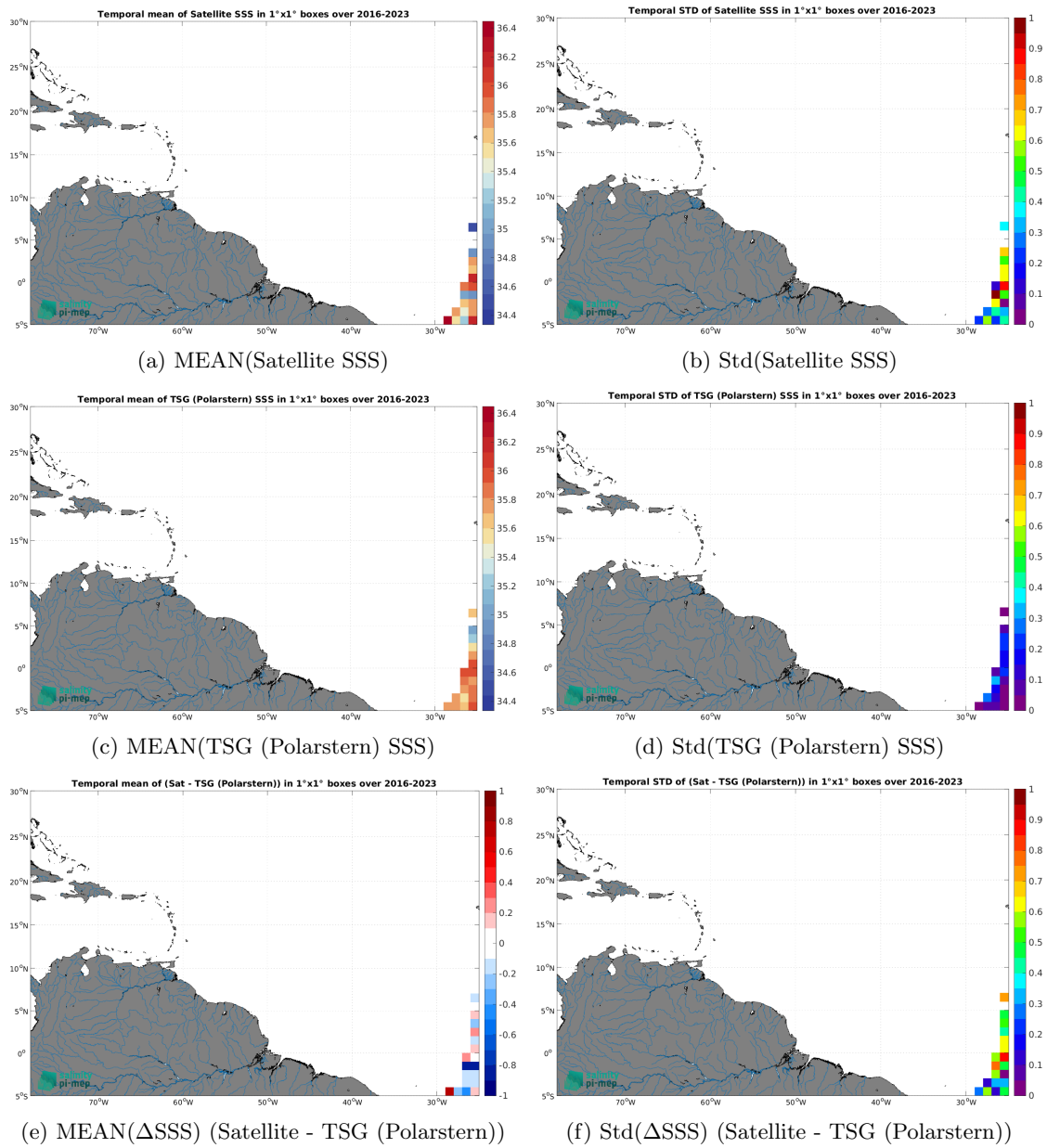
Figure 7: Temporal mean (left) and Std (right) of SSS from SMAP SSS L2 v5.3 - 40 km (RSS) (top), TSG (Polarstern) (middle), and of \Delta SSS (Satellite - TSG (Polarstern)). Only match-up pairs are used to generate these maps.
