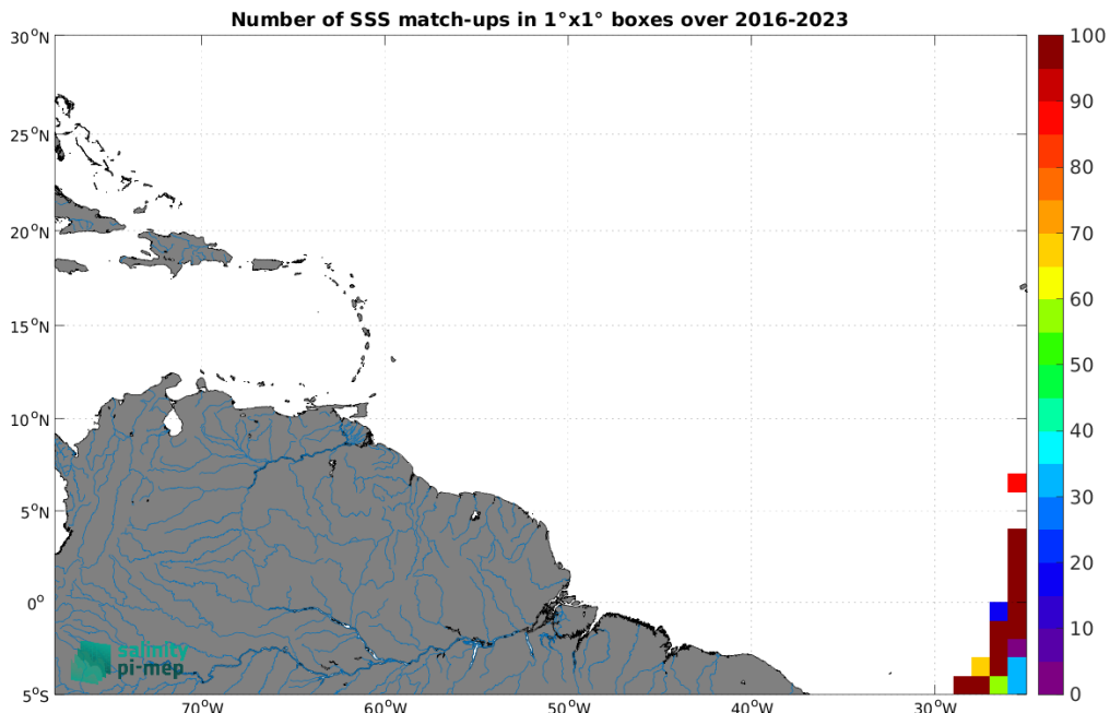
Figure 5: Number of SSS match-ups between TSG (Polarstern) SSS and the SMAP SSS L2 v5.3 - 40 km (RSS) SSS product for the Amazon and Orinoco river plumes Pi-MEP region over 1^\circ \times 1^\circ boxes and for the full satellite product period.
