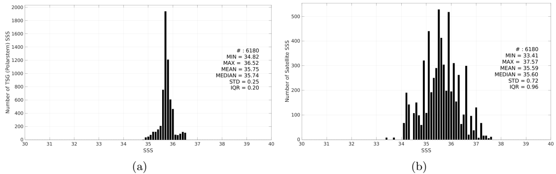
Figure 3: Histograms of SSS from TSG (Polarstern) (a) and SMAP SSS L2 v5.3 - 40 km (RSS) (b) considering all match-up pairs per bins of 0.1 over the Amazon and Orinoco river plumes Pi-MEP region and for the full satellite product period.
