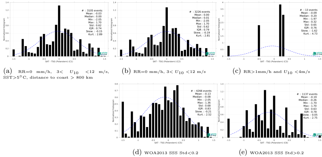
Figure 15: Normalized histogram of \Delta\text{SSS} (SMAP SSS L2 v5.3 - 40 km (RSS) - TSG (Polarstern)) for 5 different subdatasets corresponding to: RR=0 mm/h, 3 < U_{10} < 12 m/s, SST > 5°C, distance to coast > 800 km (a), RR=0 mm/h, 3 < U_{10} < 12 m/s (b), RR > 1mm/h and U_{10} < 4 m/s (c), WOA2013 SSS Std < 0.2 (d), WOA2013 SSS Std > 0.2 (e).
