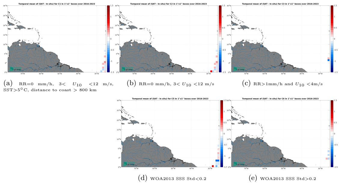
Figure 14: Temporal mean gridded over spatial boxes of size 1^\circ \times 1^\circ of \Delta SSS (SMAP SSS L2 v5.3 - 40 km (RSS) - TSG (Polarstern)) for 5 different subdatasets corresponding to: RR=0 mm/h, 3 < U_{10} < 12 m/s, SST > 5°C, distance to coast > 800 km (a), RR=0 mm/h, 3 < U_{10} < 12 m/s (b), RR > 1mm/h and U_{10} < 4 m/s (c), WOA2013 SSS Std < 0.2 (d), WOA2013 SSS Std > 0.2 (e).
