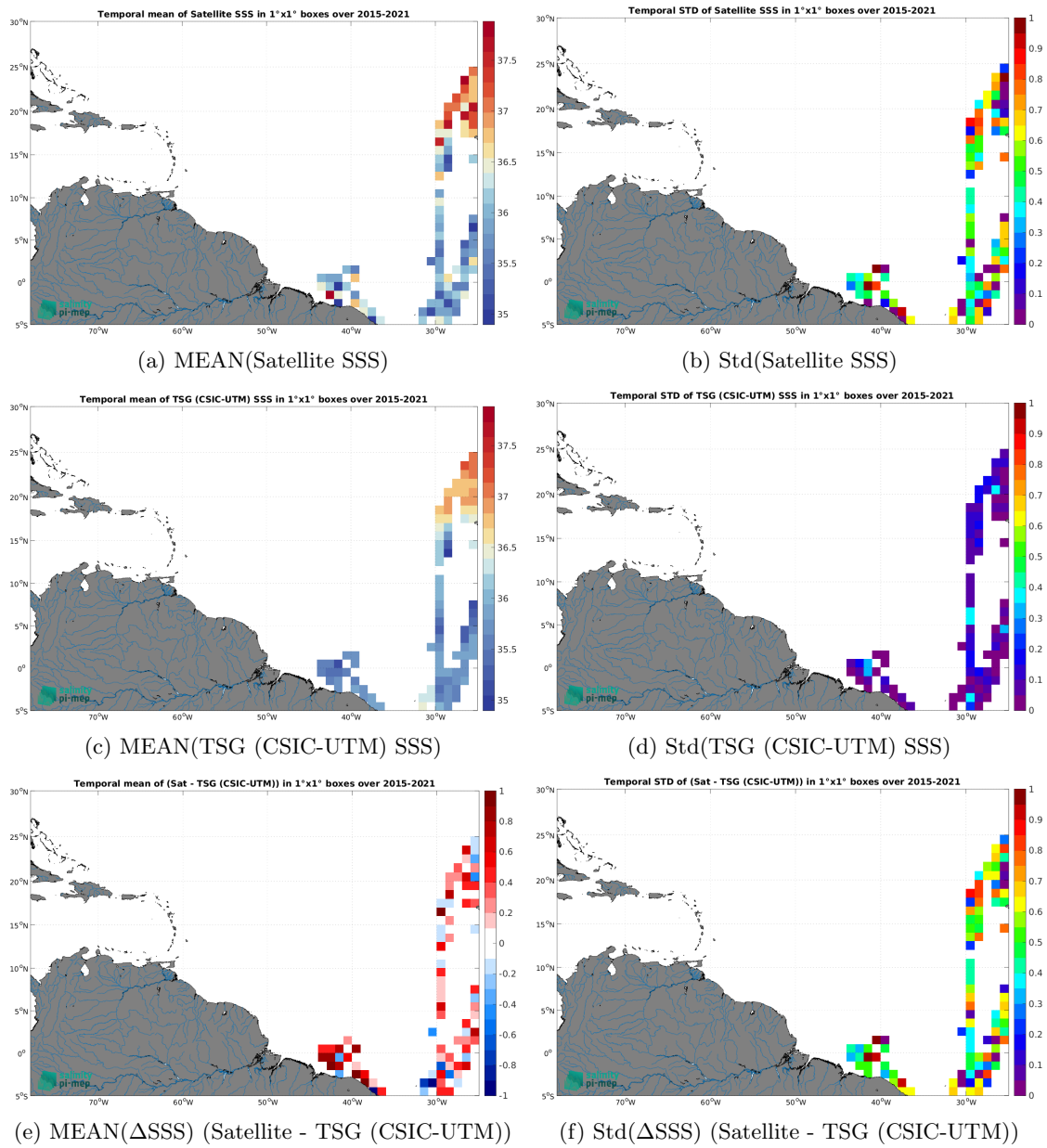
Figure 7: Temporal mean (left) and Std (right) of SSS from SMAP SSS L2 v5.3 - 40 km (RSS) (top), TSG (CSIC-UTM) (middle), and of \Delta SSS (Satellite - TSG (CSIC-UTM)). Only match-up pairs are used to generate these maps.
