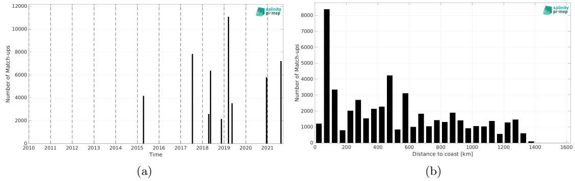
Figure 2: Number of match-ups between TSG (CSIC-UTM) and SMAP SSS L2 v5.3 - 40 km (RSS) SSS as a function of time (a) and as function of the distance to coast (b) over the Amazon and Orinoco river plumes Pi-MEP region and for the full satellite product period.
