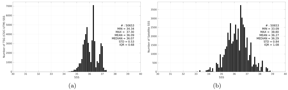
Figure 3: Histograms of SSS from TSG (CSIC-UTM) (a) and SMAP SSS L2 v5.3 - 40 km (RSS) (b) considering all match-up pairs per bins of 0.1 over the Amazon and Orinoco river plumes Pi-MEP region and for the full satellite product period.
