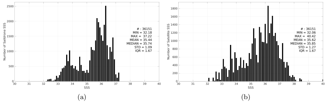
Figure 3: Histograms of SSS from Saildrone (a) and SMAP SSS L2 v5.3 - 40 km (RSS) (b) considering all match-up pairs per bins of 0.1 over the Amazon and Orinoco river plumes Pi-MEP region and for the full satellite product period.
