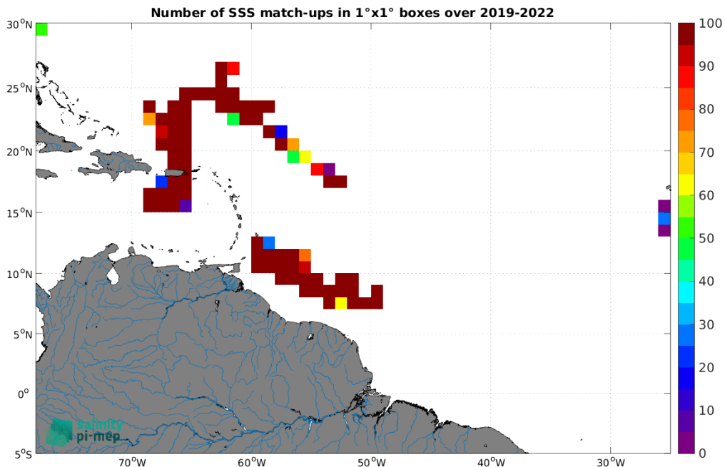
Figure 5: Number of SSS match-ups between Saildrone SSS and the SMAP SSS L2 v5.3 - 40 km (RSS) SSS product for the Amazon and Orinoco river plumes Pi-MEP region over 1^\circ \times 1^\circ boxes and for the full satellite product period.
