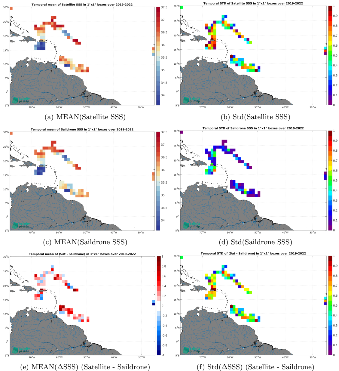
Figure 7: Temporal mean (left) and Std (right) of SSS from SMAP SSS L2 v5.3 - 40 km (RSS) (top), Saildrone (middle), and of \Delta SSS (Satellite - Saildrone). Only match-up pairs are used to generate these maps.
