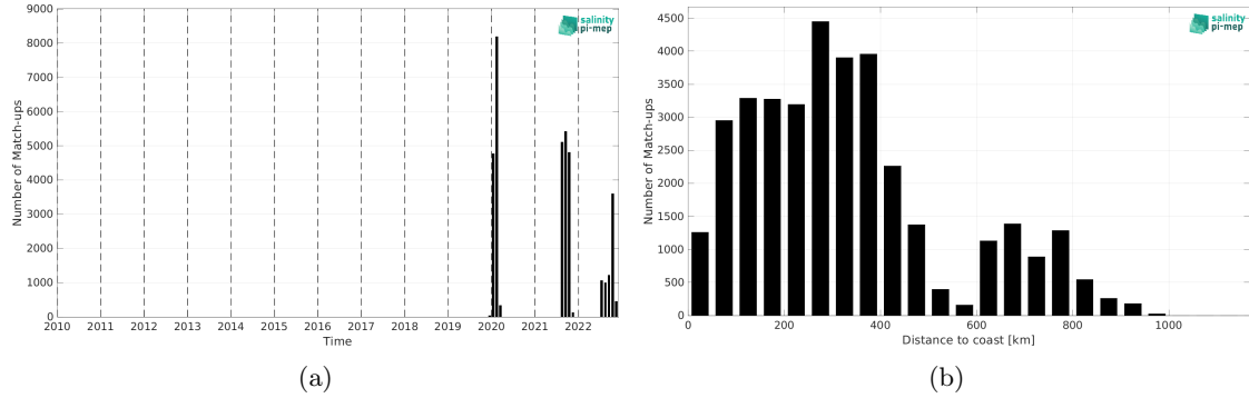
Figure 2: Number of match-ups between Saildrone and SMAP SSS L2 v5.3 - 40 km (RSS) SSS as a function of time (a) and as function of the distance to coast (b) over the Amazon and Orinoco river plumes Pi-MEP region and for the full satellite product period.
