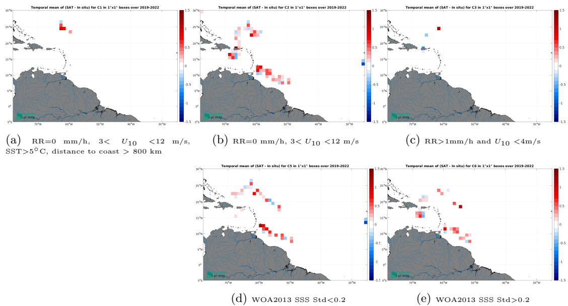
Figure 14: Temporal mean gridded over spatial boxes of size 1^\circ \times 1^\circ of \Delta\text{SSS} (SMAP SSS L2 v5.3 - 40 km (RSS) - Sailability) for 5 different subdatasets corresponding to:RR=0 mm/h, 3 < U_{10} < 12 m/s, SST>5°C, distance to coast > 800 km (a), RR=0 mm/h, 3 < U_{10} < 12 m/s (b), RR>1mm/h and U_{10} < 4 m/s (c), WOA2013 SSS Std<0.2 (d), WOA2013 SSS Std>0.2 (e).
