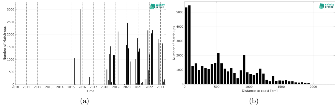
Figure 1: Number of match-ups between TSG (SAMOS) and SMAP SSS L2 v5 - 40 km (RSS) SSS as a function of time (a) and as function of the distance to coast (b) over the Amazon and Orinoco river plumes Pi-MEP region and for the full satellite product period.
