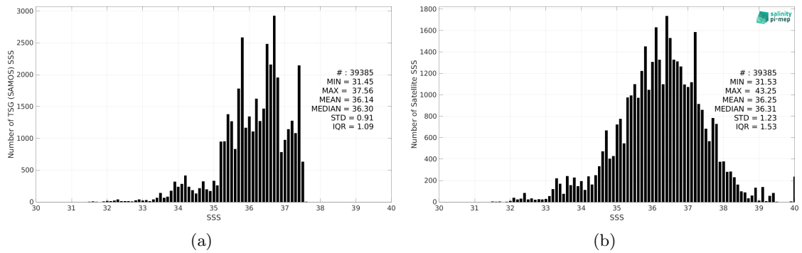
Figure 2: Histograms of SSS from TSG (SAMOS) (a) and SMAP SSS L2 v5 - 40 km (RSS) (b) considering all match-up pairs per bins of 0.1 over the Amazon and Orinoco river plumes Pi-MEP region and for the full satellite product period.
