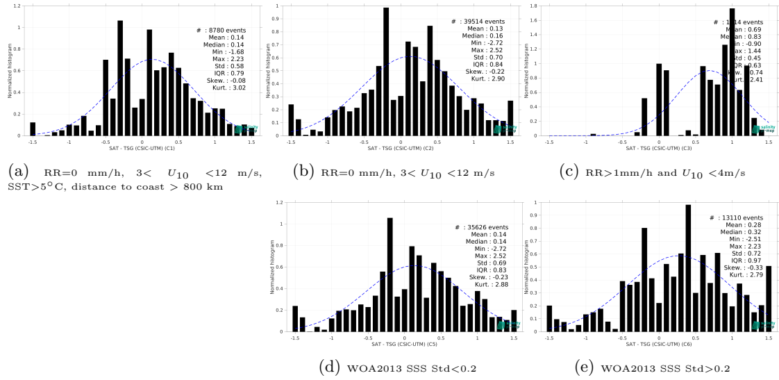
Figure 13: Normalized histogram of \Delta\text{SSS} (SMAP SSS L2 v5 - 40 km (RSS) - TSG (CSIC-UTM)) for 5 different subdatasets corresponding to: RR=0 mm/h, 3 < U_{10} < 12 m/s, SST>5°C, distance to coast > 800 km (a), RR=0 mm/h, 3 < U_{10} < 12 m/s (b), RR>1mm/h and U_{10} < 4 m/s (c), WOA2013 SSS Std<0.2 (d), WOA2013 SSS Std>0.2 (e).
