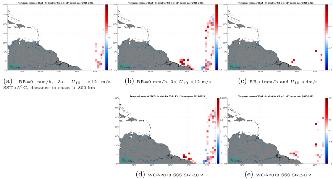
Figure 12: Temporal mean gridded over spatial boxes of size 1^\circ \times 1^\circ of \Delta SSS (SMAP SSS L2 v5 - 40 km (RSS) - TSG (CSIC-UTM)) for 5 different subdatasets corresponding to:RR=0 mm/h, 3 < U_{10} < 12 m/s, SST >5^\circ\text{C} , distance to coast > 800 km (a), RR=0 mm/h, 3 < U_{10} < 12 m/s (b), RR >1 mm/h and U_{10} < 4 m/s (c), WOA2013 SSS Std <0.2 (d), WOA2013 SSS Std >0.2 (e).
