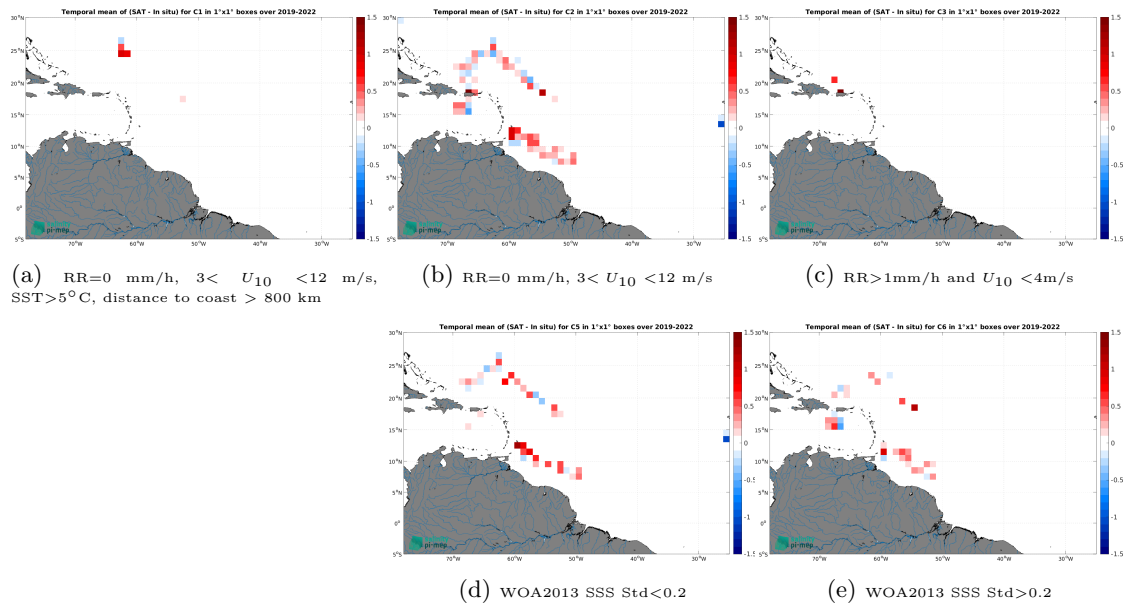
Figure 12: Temporal mean gridded over spatial boxes of size 1^\circ \times 1^\circ of \Delta SSS (SMAP SSS L2 v5 - 40 km (RSS) - Salldrone) for 5 different subdatasets corresponding to:RR=0 mm/h, 3 < U_{10} < 12 m/s, SST >5^\circ\text{C} , distance to coast > 800 km (a), RR=0 mm/h, 3 < U_{10} < 12 m/s (b), RR >1 mm/h and U_{10} < 4 m/s (c), WOA2013 SSS Std <0.2 (d), WOA2013 SSS Std >0.2 (e).
