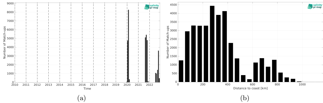
Figure 1: Number of match-ups between Saildrone and SMAP SSS L2 v5 - 40 km (RSS) SSS as a function of time (a) and as function of the distance to coast (b) over the Amazon and Orinoco river plumes Pi-MEP region and for the full satellite product period.
