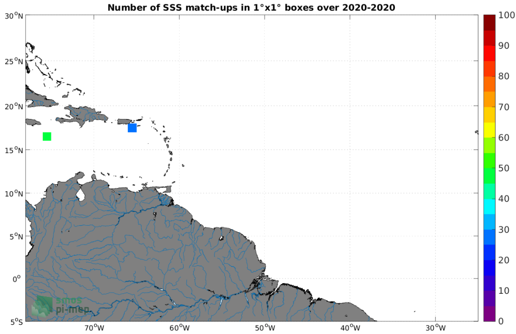
Figure 3: Number of SSS match-ups between Surface drifters SSS and the SMAP SSS L2 v5 - 40 km (RSS) SSS product for the Amazon and Orinoco river plumes Pi-MEP region over 1^\circ \times 1^\circ boxes and for the full satellite product period.
