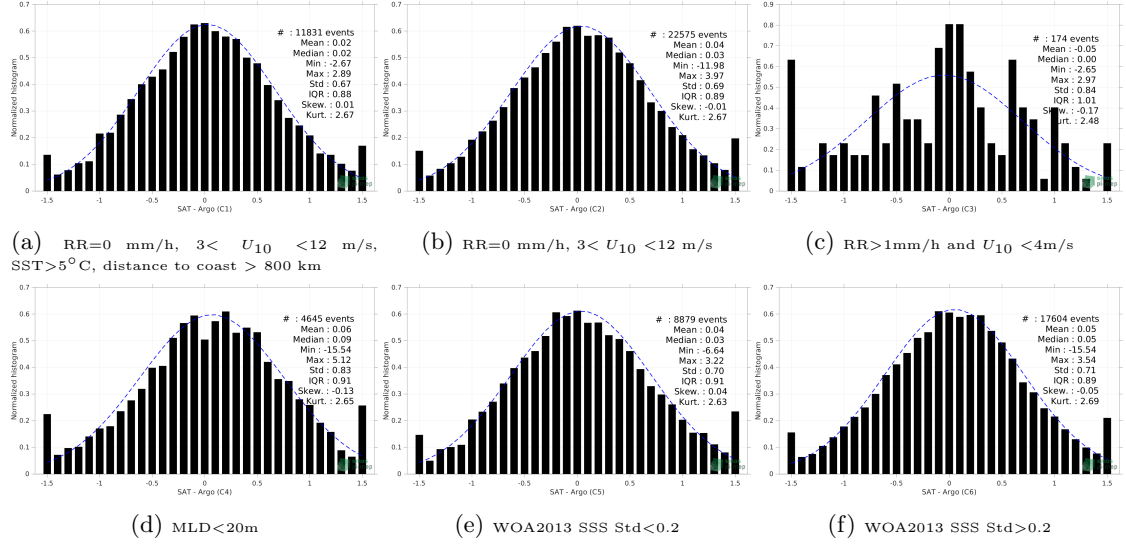
Figure 13: Normalized histogram of \Delta SSS (SMAP SSS L2 v5 - 40 km (RSS) - Argo) for 6 different subdatasets corresponding to: RR=0 mm/h, 3 < U_{10} < 12 m/s, SST > 5°C, distance to coast > 800 km (a), RR=0 mm/h, 3 < U_{10} < 12 m/s (b), RR > 1mm/h and U_{10} < 4 m/s (c), MLD < 20m (d), WOA2013 SSS Std < 0.2 (e), WOA2013 SSS Std > 0.2 (f).
