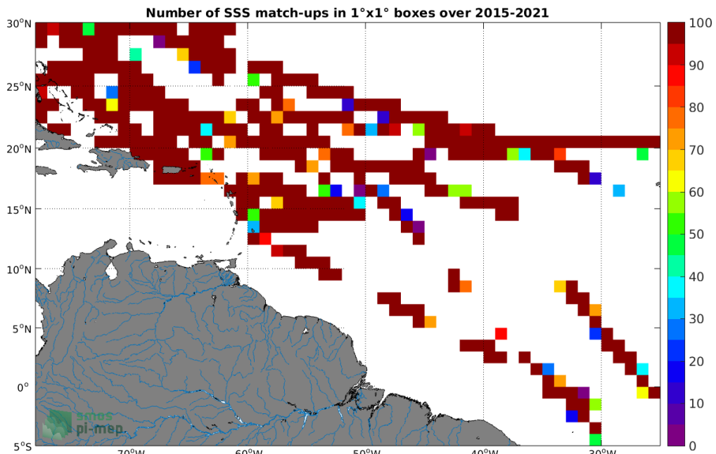
Figure 4: Number of SSS match-ups between TSG (SAMOS) SSS and the SMAP SSS L2 v4 (RSS) SSS product for the Amazon and Orinoco river plumes Pi-MEP region over 1^\circ \times 1^\circ boxes and for the full satellite product period.
