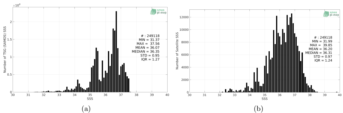
Figure 2: Histograms of SSS from TSG (SAMOS) (a) and SMAP SSS L2 v4 (RSS) (b) considering all match-up pairs per bins of 0.1 over the Amazon and Orinoco river plumes Pi-MEP region and for the full satellite product period.
