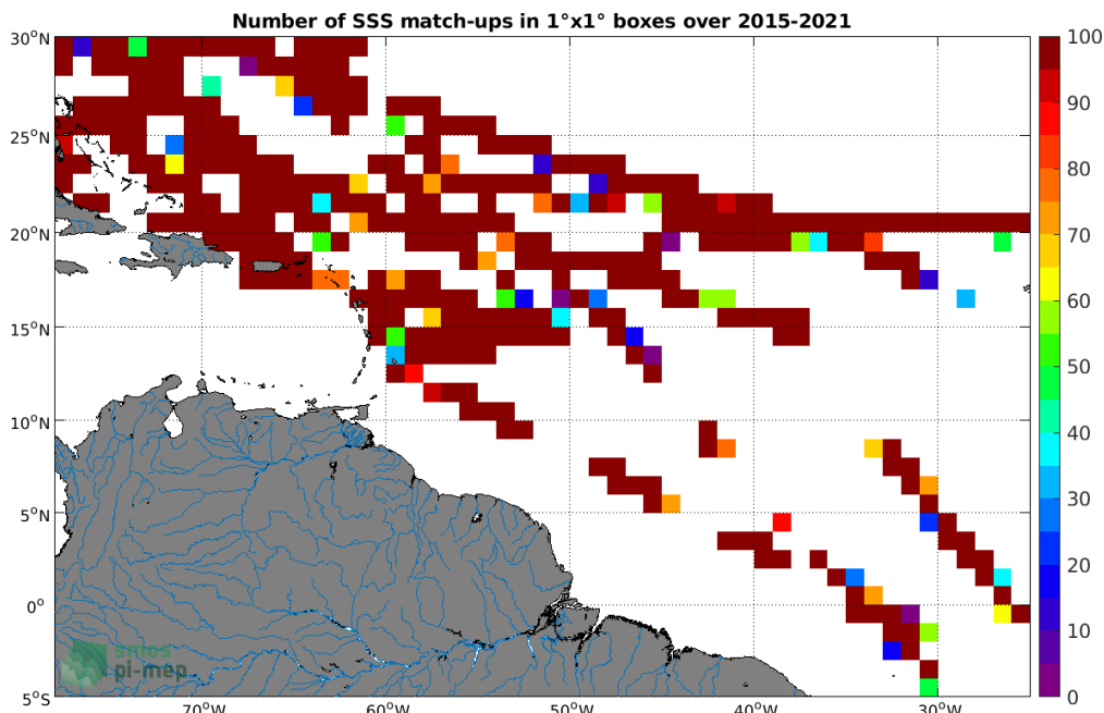
Figure 4: Number of SSS match-ups between TSG (SAMOS) SSS and the SMAP SSS L2 v4 (RSS) SSS product for the Amazon and Orinoco river plumes Pi-MEP region over 1^{\circ} \times 1^{\circ} boxes and for the full satellite product period.
