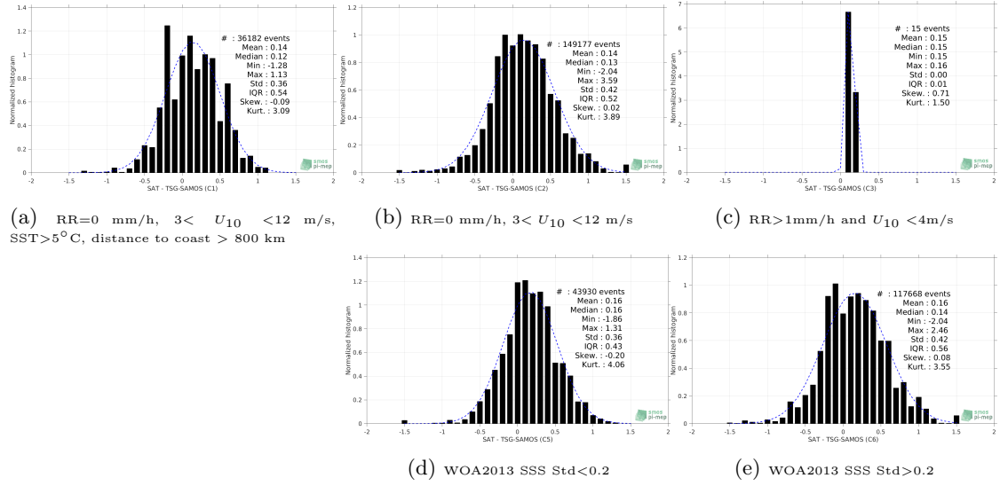
Figure 13: Normalized histogram of \Delta SSS (SMAP-L2-RSS-V4 - TSG-SAMOS) for 5 different subdatasets corresponding to: RR=0 mm/h, 3 < U_{10} < 12 m/s, SST > 5°C, distance to coast > 800 km (a), RR=0 mm/h, 3 < U_{10} < 12 m/s (b), RR > 1mm/h and U_{10} < 4 m/s (c), WOA2013 SSS Std < 0.2 (d), WOA2013 SSS Std > 0.2 (e).
