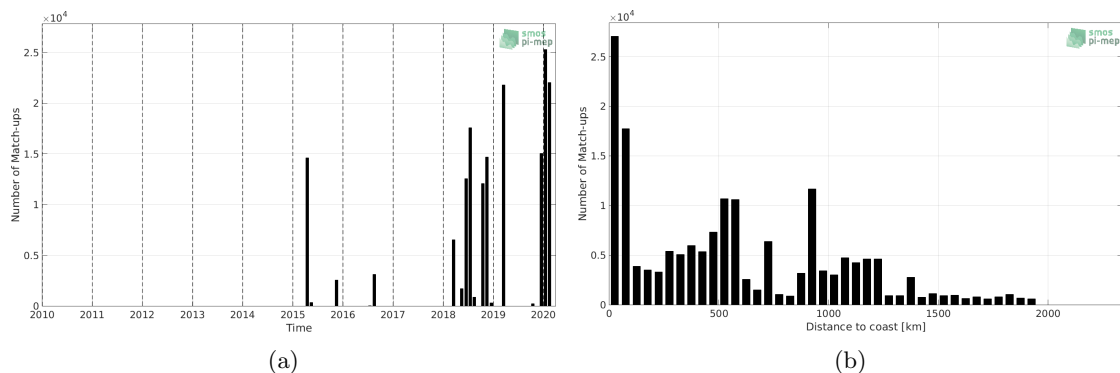
Figure 1: Number of match-ups between TSG-SAMOS and SMAP-L2-RSS-V4 SSS as a function of time (a) and as function of the distance to coast (b) over the Amazon and Orinoco river plumes Pi-MEP region and for the full satellite product period.
