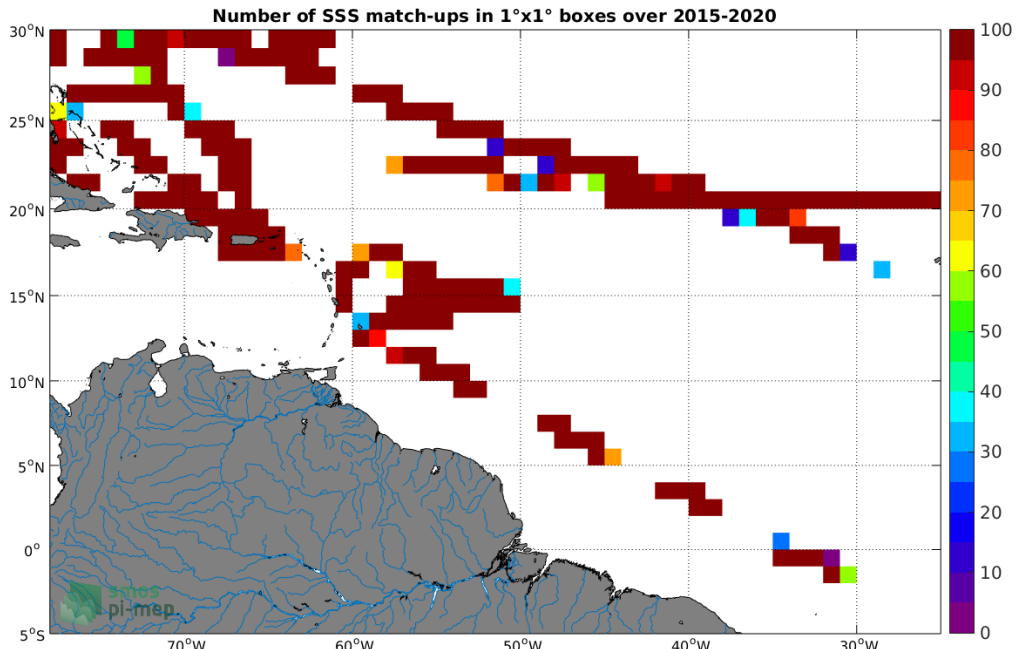
Figure 4: Number of SSS match-ups between TSG-SAMOS SSS and the SMAP-L2-RSS-V4 SSS product for the Amazon and Orinoco river plumes Pi-MEP region over 1°x1° boxes and for the full satellite product period.
