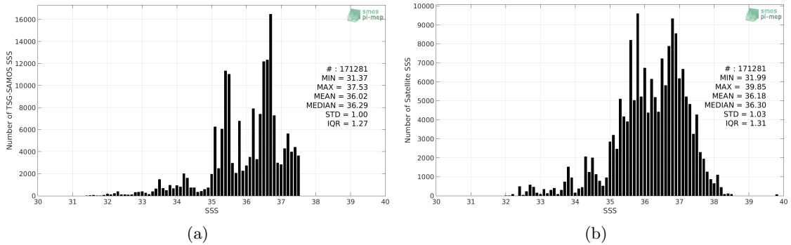
Figure 2: Histograms of SSS from TSG-SAMOS (a) and SMAP-L2-RSS-V4 (b) considering all match-up pairs per bins of 0.1 over the Amazon and Orinoco river plumes Pi-MEP region and for the full satellite product period.
