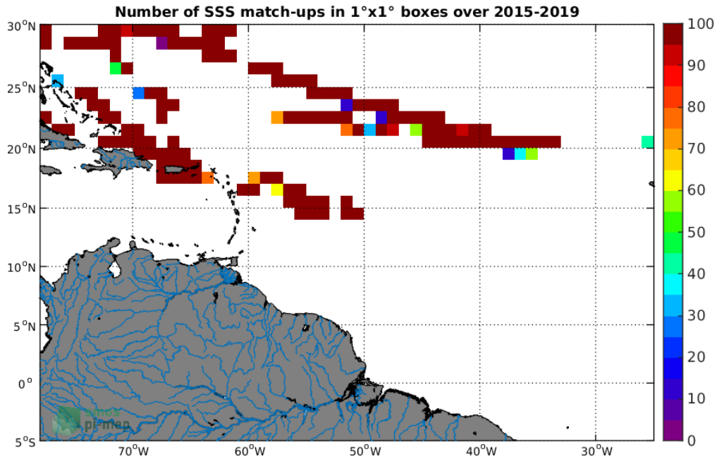
Figure 4: Number of SSS match-ups between TSG-SAMOS SSS and the SMAP-L2-RSS-V4 SSS product for the Amazon and Orinoco river plumes Pi-MEP region over 1^\circ \times 1^\circ boxes and for the full satellite product period.
