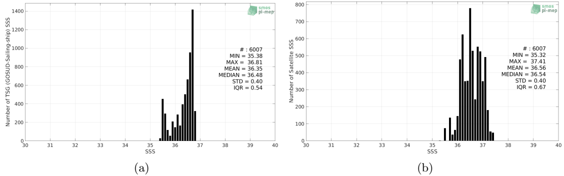
Figure 2: Histograms of SSS from TSG (GOSUD-Sailing-ship) (a) and SMAP SSS L2 v4 (RSS) (b) considering all match-up pairs per bins of 0.1 over the Amazon and Orinoco river plumes Pi-MEP region and for the full satellite product period.
