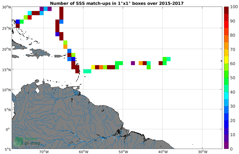
Figure 4: Number of SSS match-ups between TSG (GOSUD-Sailing-ship) SSS and the SMAP SSS L2 v4 (RSS) SSS product for the Amazon and Orinoco river plumes Pi-MEP region over 1^{\circ} \times 1^{\circ} boxes and for the full satellite product period.
