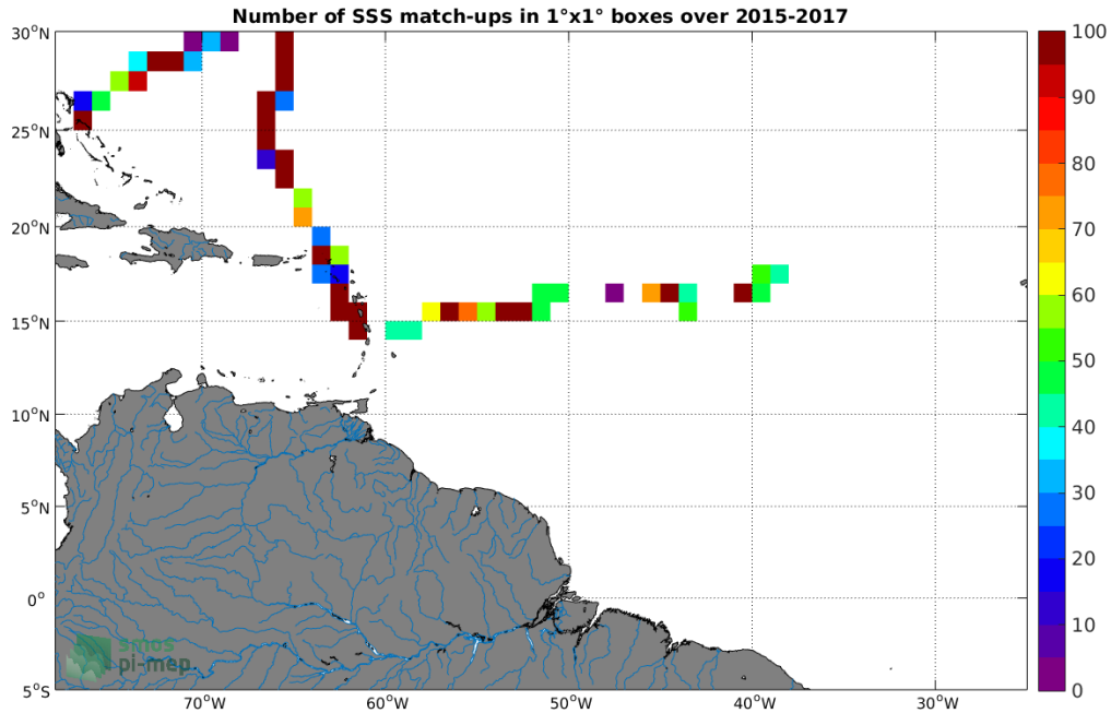
Figure 4: Number of SSS match-ups between TSG (GOSUD-Sailing-ship) SSS and the SMAP SSS L2 v4 (RSS) SSS product for the Amazon and Orinoco river plumes Pi-MEP region over 1°x1° boxes and for the full satellite product period.
