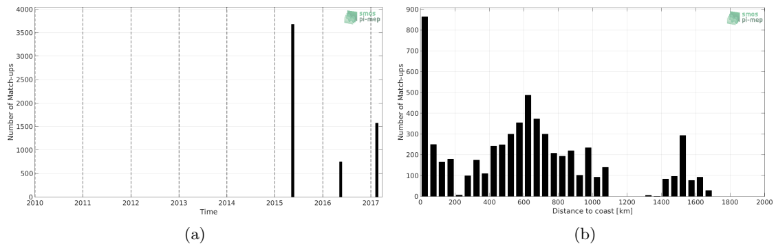
Figure 1: Number of match-ups between TSG-GOSUD-Sailing-ship and SMAP-L2-RSS-V4 SSS as a function of time (a) and as function of the distance to coast (b) over the Amazon and Orinoco river plumes Pi-MEP region and for the full satellite product period.
