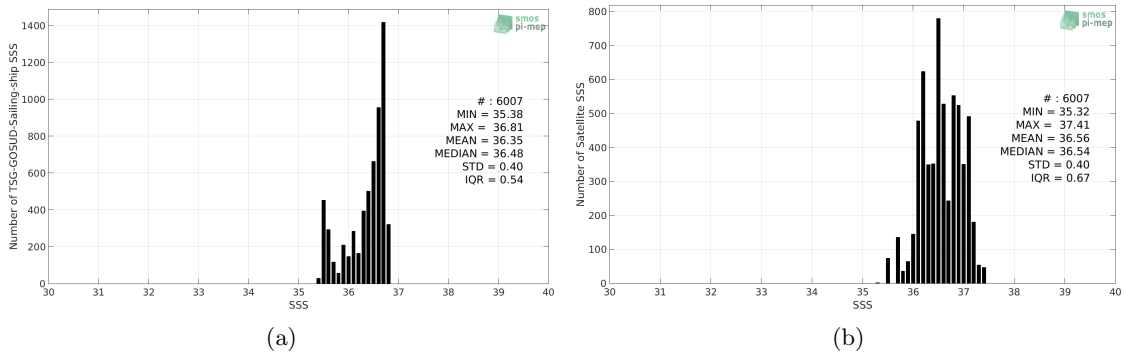
Figure 2: Histograms of SSS from TSG-GOSUD-Sailing-ship (a) and SMAP-L2-RSS-V4 (b) considering all match-up pairs per bins of 0.1 over the Amazon and Orinoco river plumes Pi-MEP region and for the full satellite product period.
