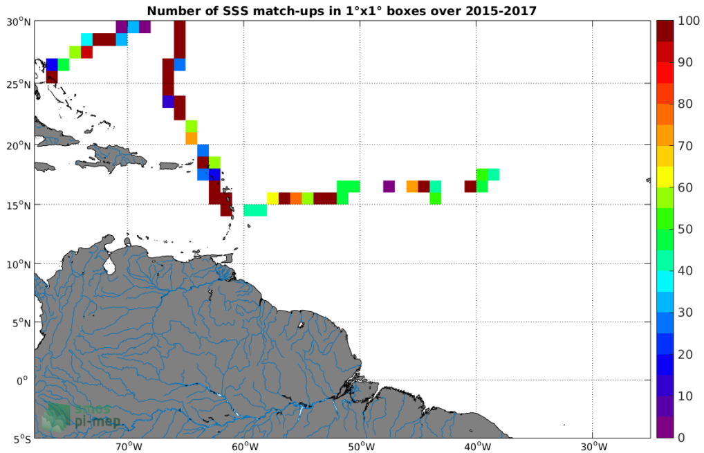
Figure 4: Number of SSS match-ups between TSG-GOSUD-Sailing-ship SSS and the SMAP-L2-RSS-V4 SSS product for the Amazon and Orinoco river plumes Pi-MEP region over 1^\circ \times 1^\circ boxes and for the full satellite product period.
