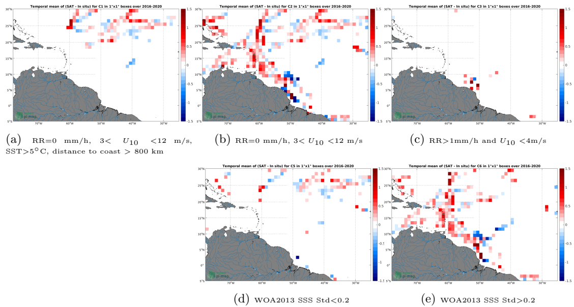
Figure 12: Temporal mean gridded over spatial boxes of size 1^\circ \times 1^\circ of \Delta SSS (SMAP SSS L2 v4 (RSS) - TSG (GOSUD-Research-vessel)) for 5 different subdatasets corresponding to: RR=0 mm/h, 3 < U_{10} < 12 m/s, SST > 5°C, distance to coast > 800 km (a), RR=0 mm/h, 3 < U_{10} < 12 m/s (b), RR > 1mm/h and U_{10} < 4 m/s (c), WOA2013 SSS Std < 0.2 (d), WOA2013 SSS Std > 0.2 (e).
