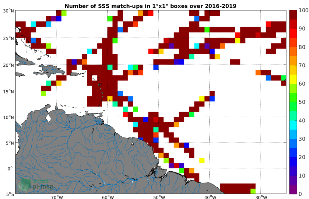
Figure 4: Number of SSS match-ups between TSG (GOSUD-Research-vessel) SSS and the SMAP SSS L2 v4 (RSS) SSS product for the Amazon and Orinoco river plumes Pi-MEP region over 1°x1° boxes and for the full satellite product period.
