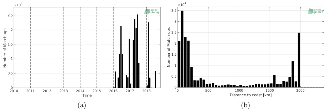
Figure 1: Number of match-ups between TSG-GOSUD-Research-vessel and SMAP-L2-RSS-V4 SSS as a function of time (a) and as function of the distance to coast (b) over the Amazon and Orinoco river plumes Pi-MEP region and for the full satellite product period.
