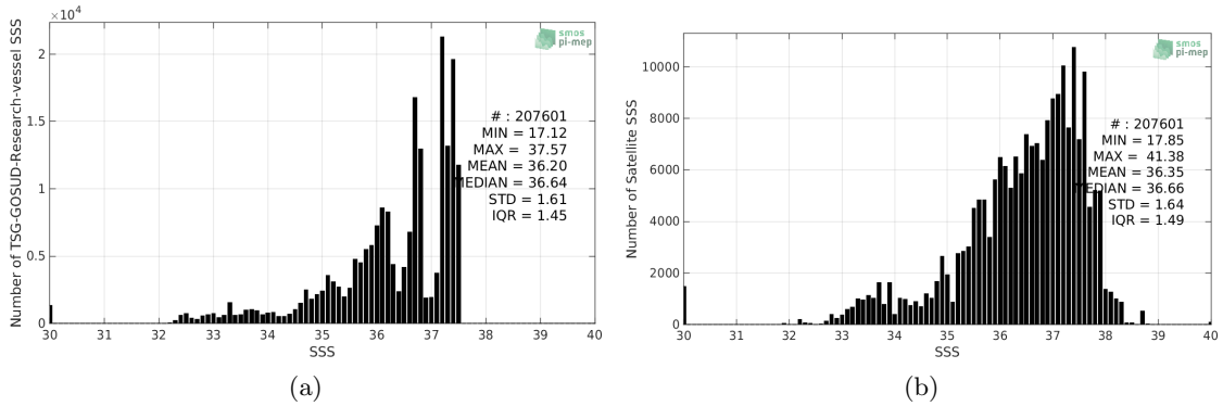
Figure 2: Histograms of SSS from TSG-GOSUD-Research-vessel (a) and SMAP-L2-RSS-V4 (b) considering all match-up pairs per bins of 0.1 over the Amazon and Orinoco river plumes Pi-MEP region and for the full satellite product period.
