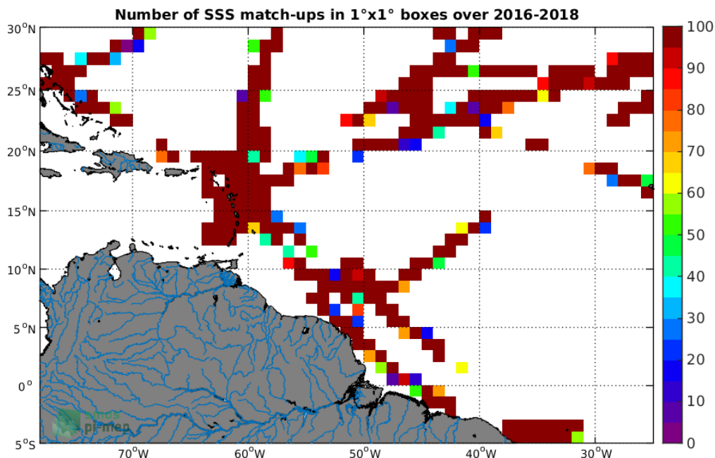
Figure 4: Number of SSS match-ups between TSG-GOSUD-Research-vessel SSS and the SMAP-L2-RSS-V4 SSS product for the Amazon and Orinoco river plumes Pi-MEP region over 1°x1° boxes and for the full satellite product period.
