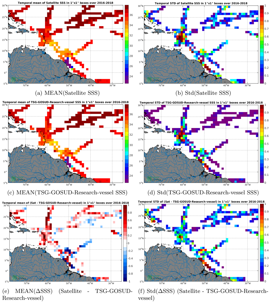
Figure 6: Temporal mean (left) and Std (right) of SSS from SMAP-L2-RSS-V4 (top), TSG-GOSUD-Research-vessel (middle), and of \Delta SSS (Satellite - TSG-GOSUD-Research-vessel). Only match-up pairs are used to generate these maps.
