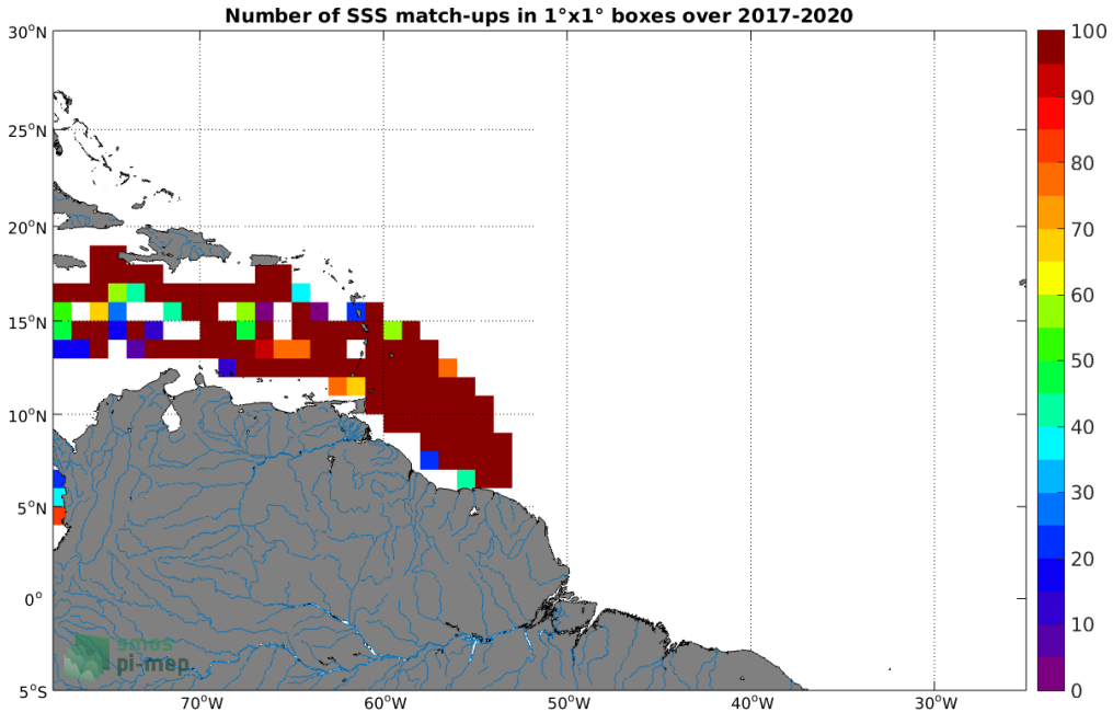
Figure 3: Number of SSS match-ups between Surface drifters SSS and the SMAP SSS L2 v4 (RSS) SSS product for the Amazon and Orinoco river plumes Pi-MEP region over 1°x1° boxes and for the full satellite product period.
