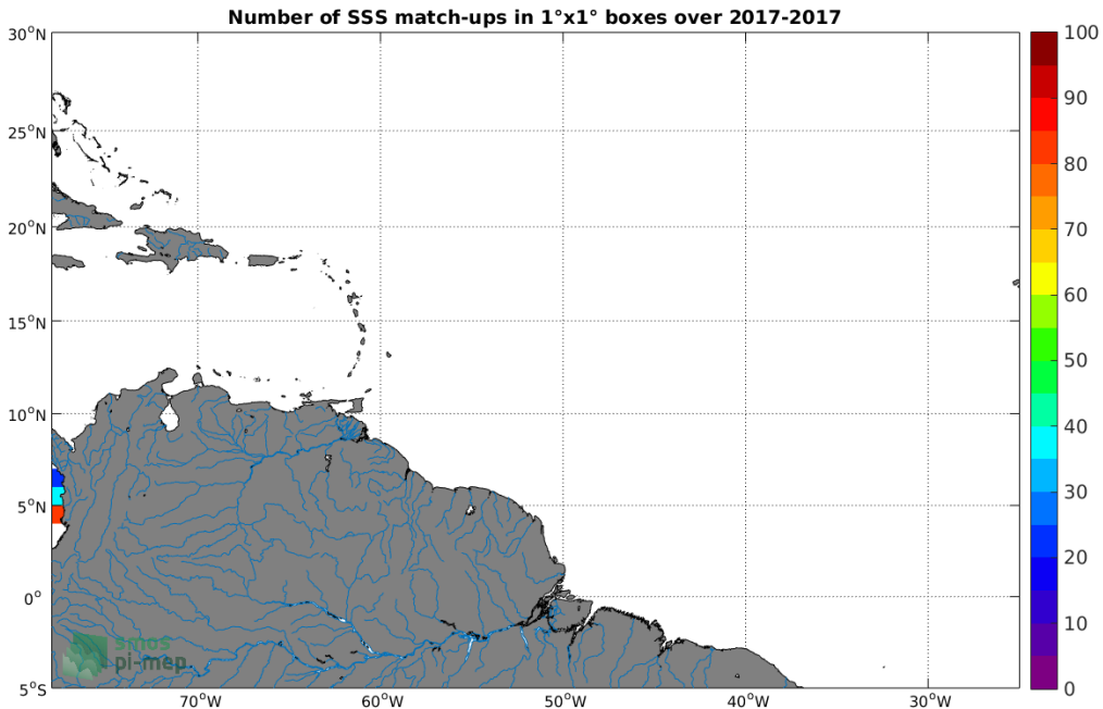
Figure 3: Number of SSS match-ups between Surface drifters SSS and the SMAP SSS L2 v4 (RSS) SSS product for the Amazon and Orinoco river plumes Pi-MEP region over 1^{\circ} \times 1^{\circ} boxes and for the full satellite product period.
