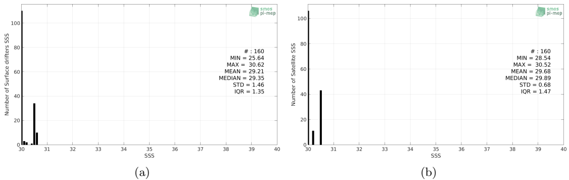
Figure 2: Histograms of SSS from Surface drifters (a) and SMAP-L2-RSS-V4 (b) considering all match-up pairs per bins of 0.1 over the Amazon and Orinoco river plumes Pi-MEP region and for the full satellite product period.
