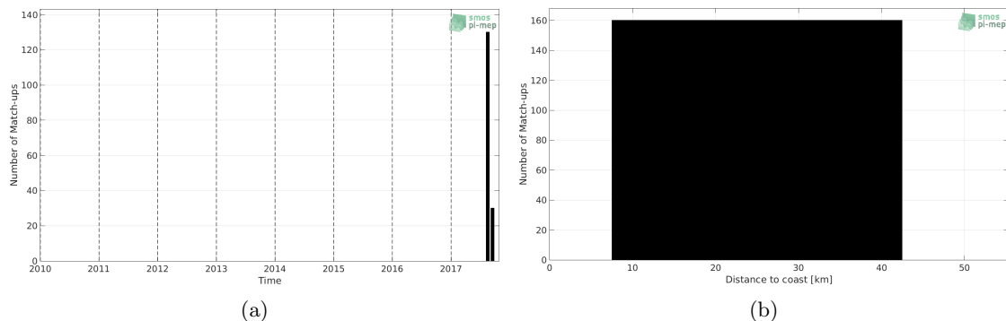
Figure 1: Number of match-ups between Surface drifters and SMAP-L2-RSS-V4 SSS as a function of time (a) and as function of the distance to coast (b) over the Amazon and Orinoco river plumes Pi-MEP region and for the full satellite product period.
