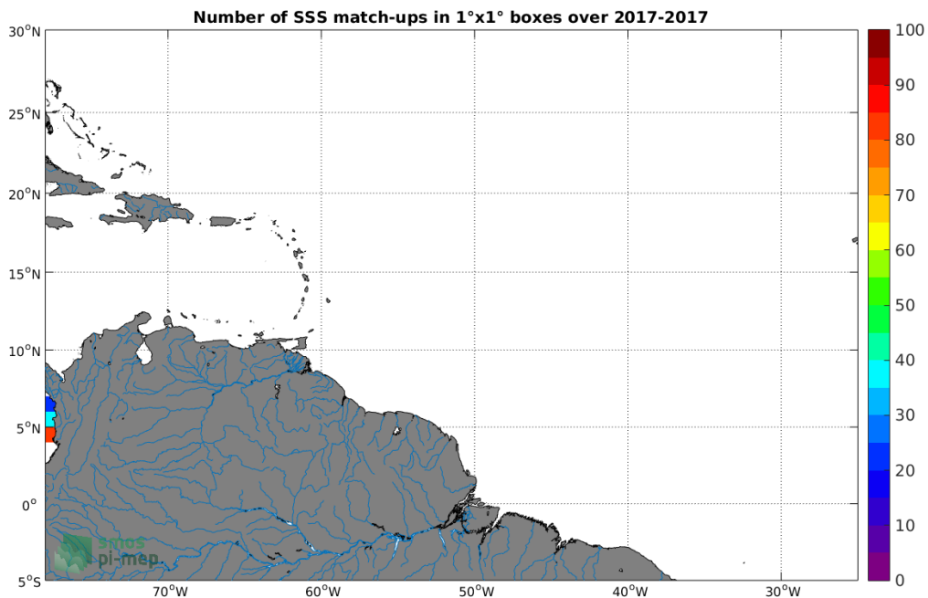
Figure 3: Number of SSS match-ups between Surface drifters SSS and the SMAP-L2-RSS-V4 SSS product for the Amazon and Orinoco river plumes Pi-MEP region over 1°x1° boxes and for the full satellite product period.
