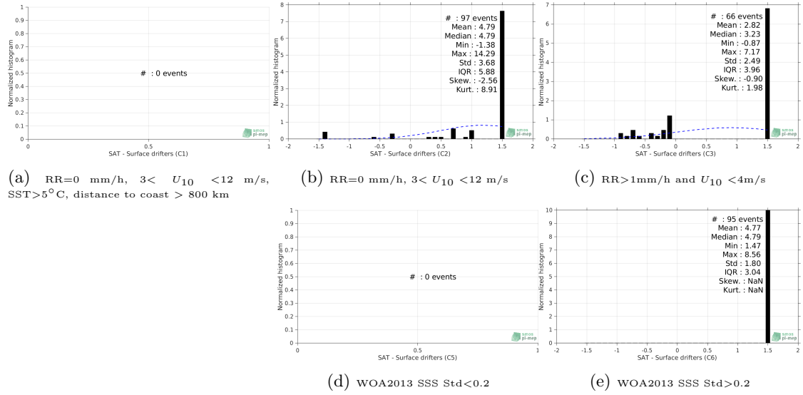
Figure 12: Normalized histogram of \Delta\text{SSS} (SMAP-L2-RSS-V4 - Surface drifters) for 5 different subdatasets corresponding to: RR=0 mm/h, 3 < U_{10} < 12 m/s, SST > 5^\circ\text{C} , distance to coast > 800 km (a), RR=0 mm/h, 3 < U_{10} < 12 m/s (b), RR > 1\text{mm/h} and U_{10} < 4\text{m/s} (c), WOA2013 SSS Std < 0.2 (d), WOA2013 SSS Std > 0.2 (e).
