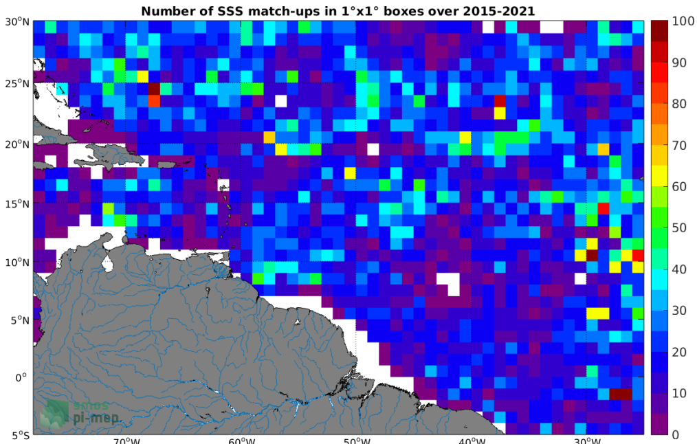
Figure 4: Number of SSS match-ups between Argo SSS and the SMAP SSS L2 v4 (RSS) SSS product for the Amazon and Orinoco river plumes Pi-MEP region over 1^\circ \times 1^\circ boxes and for the full satellite product period.
