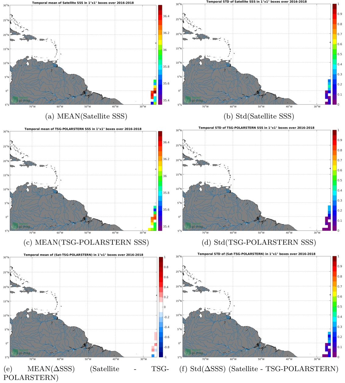
Figure 6: Temporal mean (left) and Std (right) of SSS from SMAP-L2-RSS-V3-70KM (top), TSG-POLARSTERN (middle), and of \Delta SSS (Satellite - TSG-POLARSTERN). Only match-up pairs are used to generate these maps.
