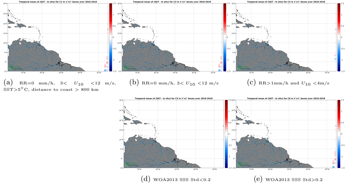
Figure 12: Temporal mean gridded over spatial boxes of size 1^\circ \times 1^\circ of \Delta SSS (SMAP-L2-RSS-V3-70KM - TSG-POLARSTERN) for 5 different subdatasets corresponding to: RR=0 mm/h, 3 < U_{10} < 12 m/s, SST > 5^\circ\text{C} , distance to coast > 800 km (a), RR=0 mm/h, 3 < U_{10} < 12 m/s (b), RR > 1 mm/h and U_{10} < 4 m/s (c), WOA2013 SSS Std < 0.2 (d), WOA2013 SSS Std > 0.2 (e).
