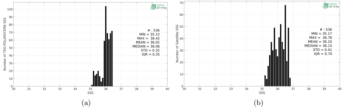
Figure 2: Histograms of SSS from TSG-POLARSTERN (a) and SMAP-L2-RSS-V3-70KM (b) considering all match-up pairs per bins of 0.1 over the Amazon and Orinoco river plumes Pi-MEP region and for the full satellite product period.
