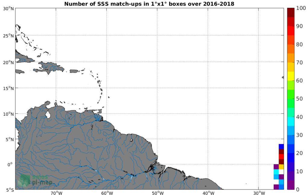
Figure 4: Number of SSS match-ups between TSG-POLARSTERN SSS and the SMAP-L2-RSS-V3-70KM SSS product for the Amazon and Orinoco river plumes Pi-MEP region over 1^\circ \times 1^\circ boxes and for the full satellite product period.
