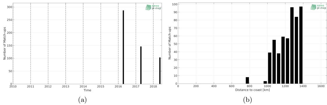
Figure 1: Number of match-ups between TSG-POLARSTERN and SMAP-L2-RSS-V3-70KM SSS as a function of time (a) and as function of the distance to coast (b) over the Amazon and Orinoco river plumes Pi-MEP region and for the full satellite product period.
