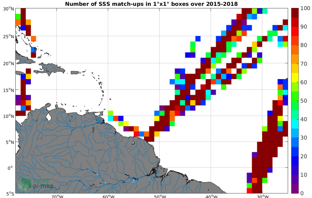
Figure 4: Number of SSS match-ups between TSG-LEGOS-DM SSS and the SMAP-L2-RSS-V3-70KM SSS product for the Amazon and Orinoco river plumes Pi-MEP region over 1^\circ \times 1^\circ boxes and for the full satellite product period.
