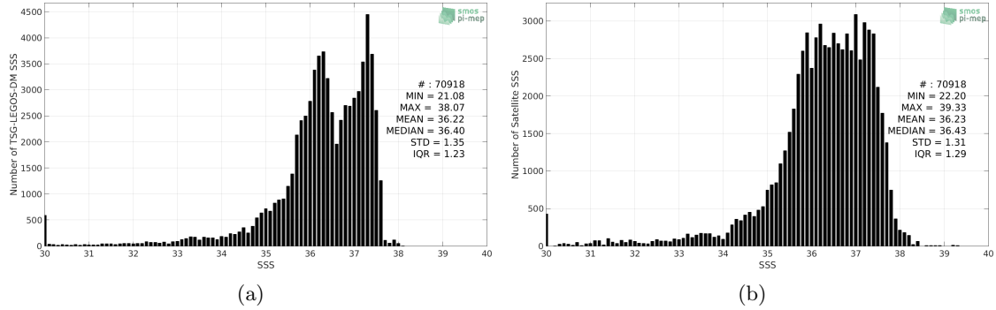
Figure 2: Histograms of SSS from TSG-LEGOS-DM (a) and SMAP-L2-RSS-V3-70KM (b) considering all match-up pairs per bins of 0.1 over the Amazon and Orinoco river plumes Pi-MEP region and for the full satellite product period.
