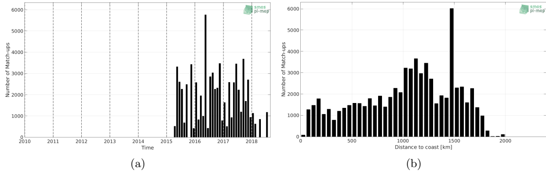
Figure 1: Number of match-ups between TSG-LEGOS-DM and SMAP-L2-RSS-V3-70KM SSS as a function of time (a) and as function of the distance to coast (b) over the Amazon and Orinoco river plumes Pi-MEP region and for the full satellite product period.
