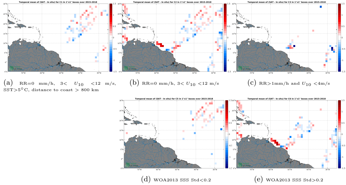
Figure 12: Temporal mean gridded over spatial boxes of size 1^\circ \times 1^\circ of \Delta SSS (SMAP-L2-RSS-V3-70KM - TSG-LEGOS-DM) for 5 different subdatasets corresponding to: RR=0 mm/h, 3 < U_{10} < 12 m/s, SST > 5^\circ C , distance to coast > 800 km (a), RR=0 mm/h, 3 < U_{10} < 12 m/s (b), RR > 1 mm/h and U_{10} < 4 m/s (c), WOA2013 SSS Std < 0.2 (d), WOA2013 SSS Std > 0.2 (e).
