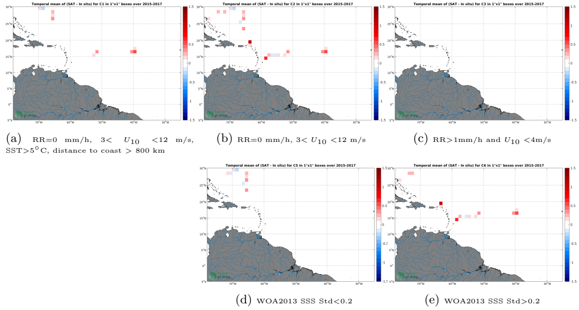
Figure 12: Temporal mean gridded over spatial boxes of size 1^\circ \times 1^\circ of \Delta SSS (SMAP-L2-RSS-V3-70KM - TSG-GOSUD-Sailing-ship) for 5 different subdatasets corresponding to: RR=0 mm/h, 3 < U_{10} < 12 m/s, SST > 5^\circ C , distance to coast > 800 km (a), RR=0 mm/h, 3 < U_{10} < 12 m/s (b), RR > 1 mm/h and U_{10} < 4 m/s (c), WOA2013 SSS Std < 0.2 (d), WOA2013 SSS Std > 0.2 (e).
