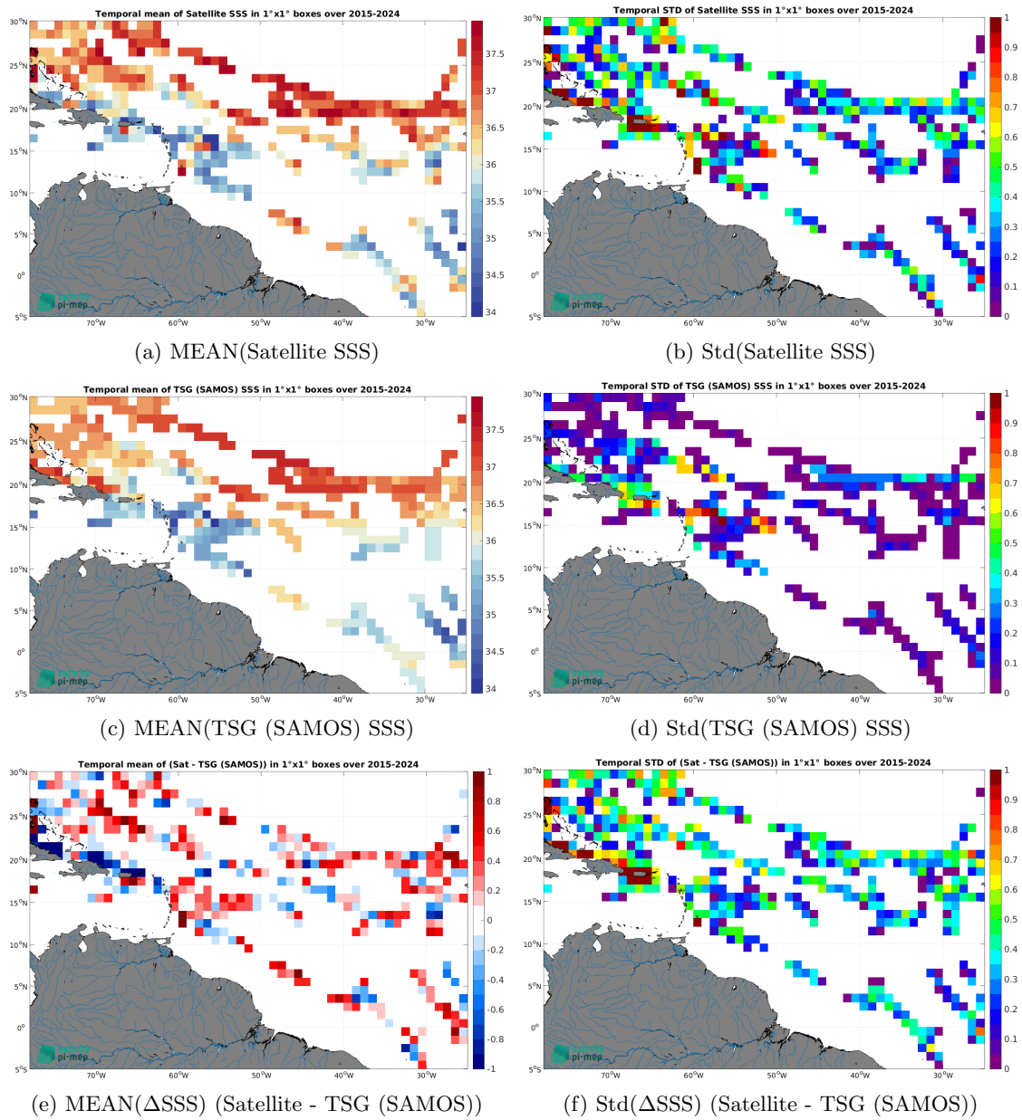
Figure 7: Temporal mean (left) and Std (right) of SSS from SMAP SSS L2 v5.0 (JPL) (top), TSG (SAMOS) (middle), and of \Delta SSS (Satellite - TSG (SAMOS)). Only match-up pairs are used to generate these maps.
