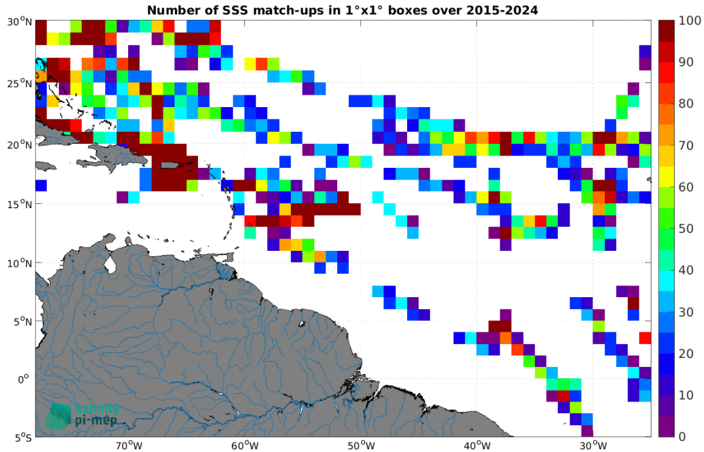
Figure 5: Number of SSS match-ups between TSG (SAMOS) SSS and the SMAP SSS L2 v5.0 (JPL) SSS product for the Amazon and Orinoco river plumes Pi-MEP region over 1^\circ \times 1^\circ boxes and for the full satellite product period.
