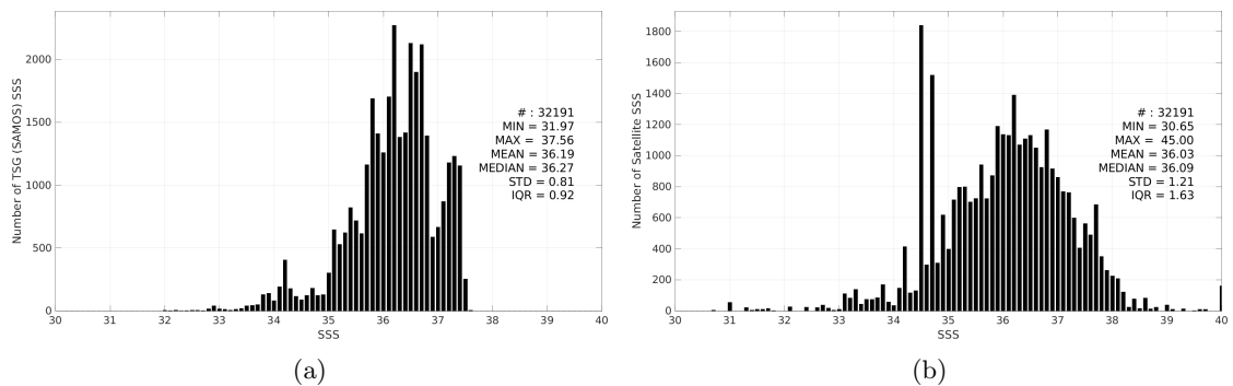
Figure 3: Histograms of SSS from TSG (SAMOS) (a) and SMAP SSS L2 v5.0 (JPL) (b) considering all match-up pairs per bins of 0.1 over the Amazon and Orinoco river plumes Pi-MEP region and for the full satellite product period.
