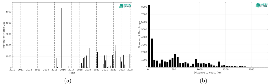
Figure 2: Number of match-ups between TSG (SAMOS) and SMAP SSS L2 v5.0 (JPL) SSS as a function of time (a) and as function of the distance to coast (b) over the Amazon and Orinoco river plumes Pi-MEP region and for the full satellite product period.
