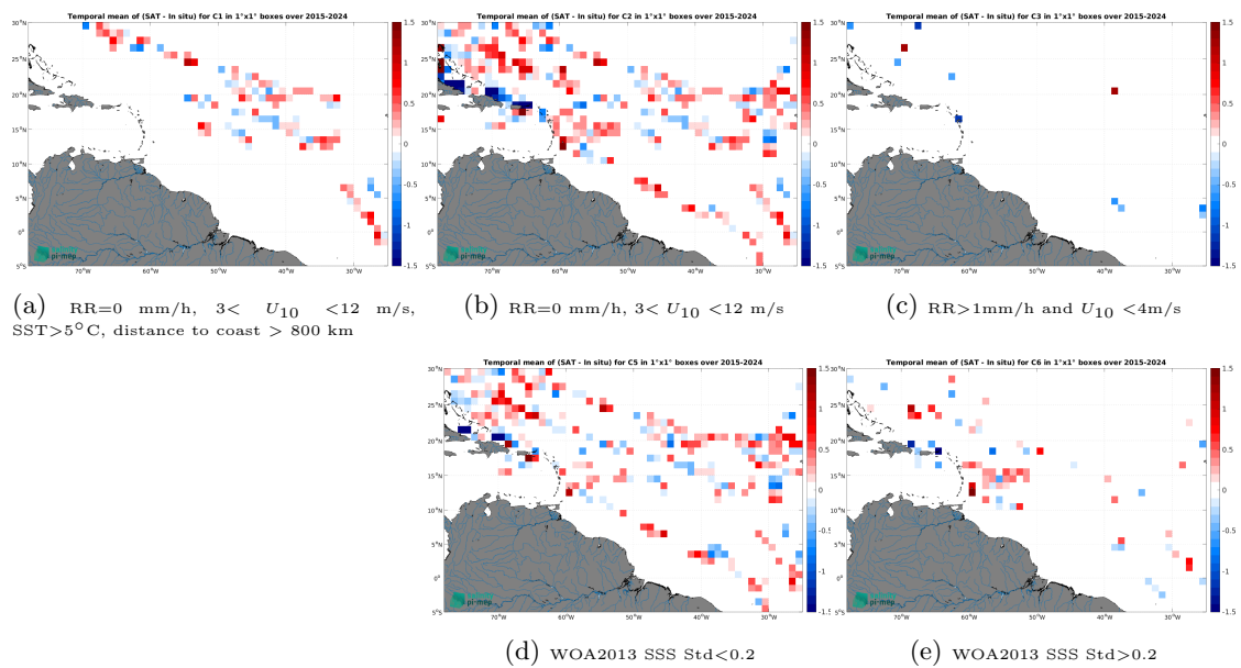
Figure 14: Temporal mean gridded over spatial boxes of size 1^\circ \times 1^\circ of \Delta SSS (SMAP SSS L2 v5.0 (JPL) - TSG (SAMOS)) for 5 different subdatasets corresponding to:RR=0 mm/h, 3 < U_{10} < 12 m/s, SST >5^\circ\text{C} , distance to coast > 800 km (a), RR=0 mm/h, 3 < U_{10} < 12 m/s (b), RR >1 mm/h and U_{10} < 4 m/s (c), WOA2013 SSS Std <0.2 (d), WOA2013 SSS Std >0.2 (e).
