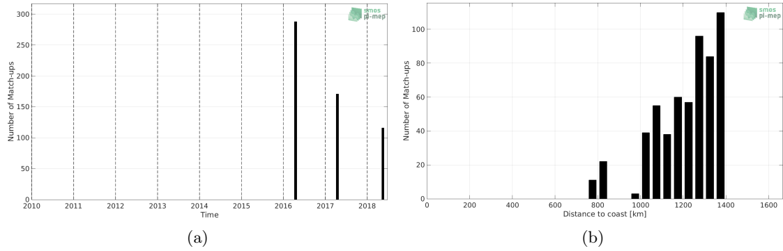
Figure 1: Number of match-ups between TSG (Polarstern) and SMAP SSS L2 v5.0 (JPL) SSS as a function of time (a) and as function of the distance to coast (b) over the Amazon and Orinoco river plumes Pi-MEP region and for the full satellite product period.
