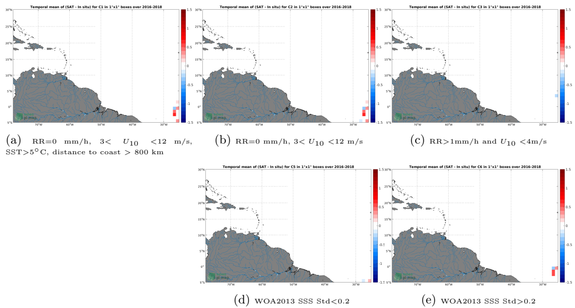
Figure 12: Temporal mean gridded over spatial boxes of size 1^\circ \times 1^\circ of \Delta SSS (SMAP SSS L2 v5.0 (JPL) - TSG (Polarstern)) for 5 different subdatasets corresponding to:RR=0 mm/h, 3 < U_{10} < 12 m/s, SST >5^\circ C, distance to coast > 800 km (a), RR=0 mm/h, 3 < U_{10} < 12 m/s (b), RR >1 mm/h and U_{10} < 4 m/s (c), WOA2013 SSS Std <0.2 (d), WOA2013 SSS Std >0.2 (e).
