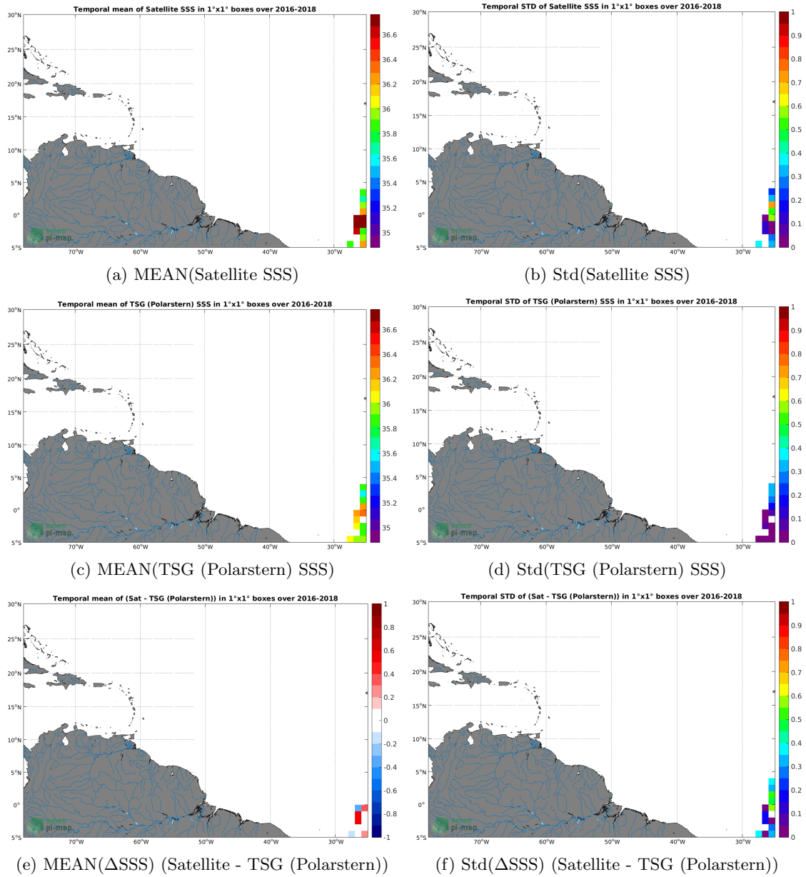
Figure 6: Temporal mean (left) and Std (right) of SSS from SMAP SSS L2 v5.0 (JPL) (top), TSG (Polarstern) (middle), and of \Delta SSS (Satellite - TSG (Polarstern)). Only match-up pairs are used to generate these maps.
