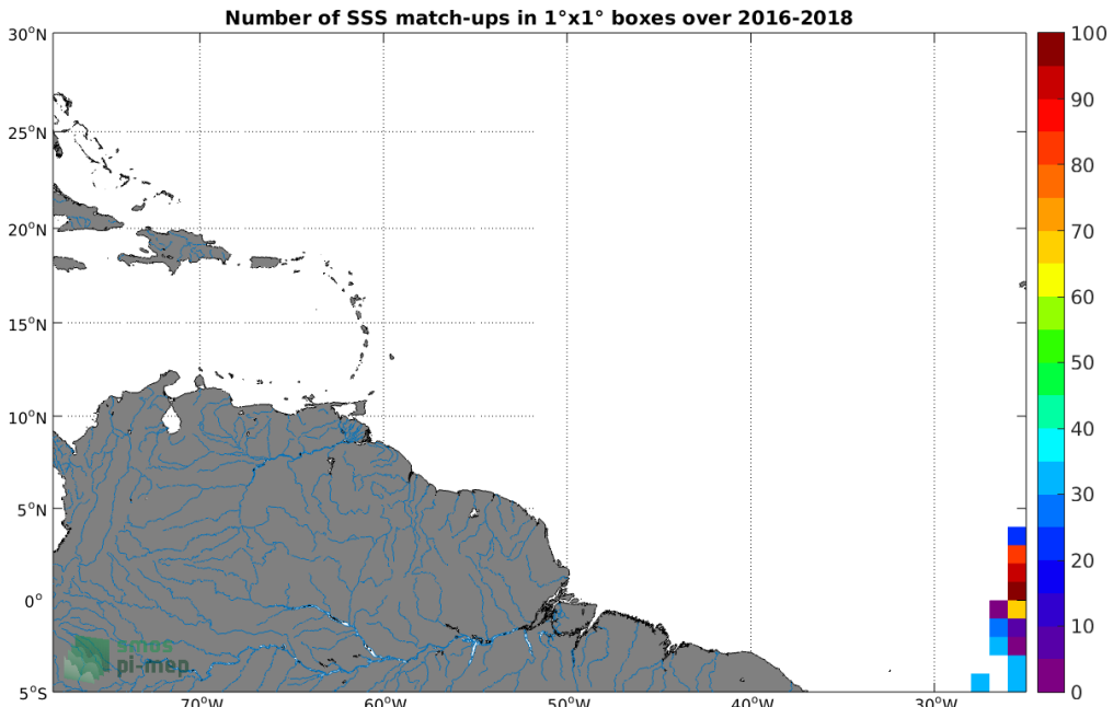
Figure 4: Number of SSS match-ups between TSG (Polarstern) SSS and the SMAP SSS L2 v5.0 (JPL) SSS product for the Amazon and Orinoco river plumes Pi-MEP region over 1^\circ \times 1^\circ boxes and for the full satellite product period.
