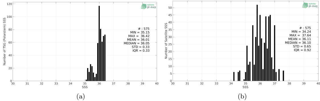
Figure 2: Histograms of SSS from TSG (Polarstern) (a) and SMAP SSS L2 v5.0 (JPL) (b) considering all match-up pairs per bins of 0.1 over the Amazon and Orinoco river plumes Pi-MEP region and for the full satellite product period.
