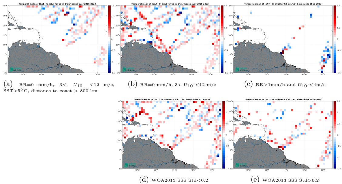
Figure 14: Temporal mean gridded over spatial boxes of size 1^\circ \times 1^\circ of \Delta\text{SSS} (SMAP SSS L2 v5.0 (JPL) - TSG (LEGOS-DM)) for 5 different subdatasets corresponding to:RR=0 mm/h, 3 < U_{10} < 12 m/s, SST >5^\circ\text{C} , distance to coast > 800 km (a), RR=0 mm/h, 3 < U_{10} < 12 m/s (b), RR >1 mm/h and U_{10} < 4 m/s (c), WOA2013 SSS Std <0.2 (d), WOA2013 SSS Std >0.2 (e).
