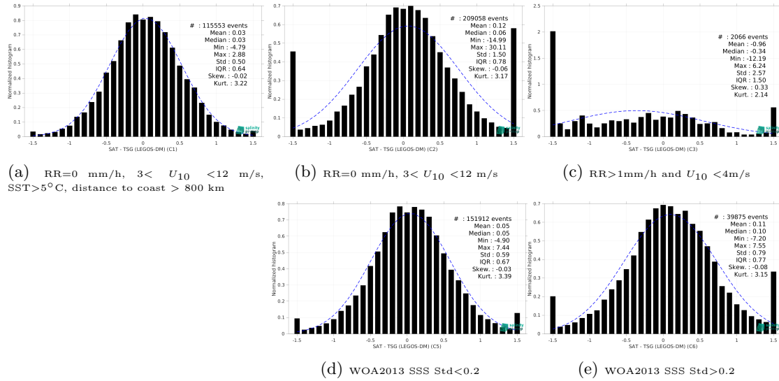
Figure 15: Normalized histogram of \Delta SSS (SMAP SSS L2 v5.0 (JPL) - TSG (LEGOS-DM)) for 5 different subdatasets corresponding to: RR=0 mm/h, 3 < U_{10} < 12 m/s, SST > 5°C, distance to coast > 800 km (a), RR=0 mm/h, 3 < U_{10} < 12 m/s (b), RR > 1mm/h and U_{10} < 4 m/s (c), WOA2013 SSS Std < 0.2 (d), WOA2013 SSS Std > 0.2 (e).
