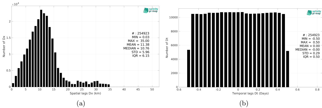
Figure 6: Histograms of the spatial (a) and temporal (b) lags between the location/time of the TSG (LEGOS-DM) measurement and the date of the corresponding SMAP SSS L2 v5.0 (JPL) SSS pixel.
