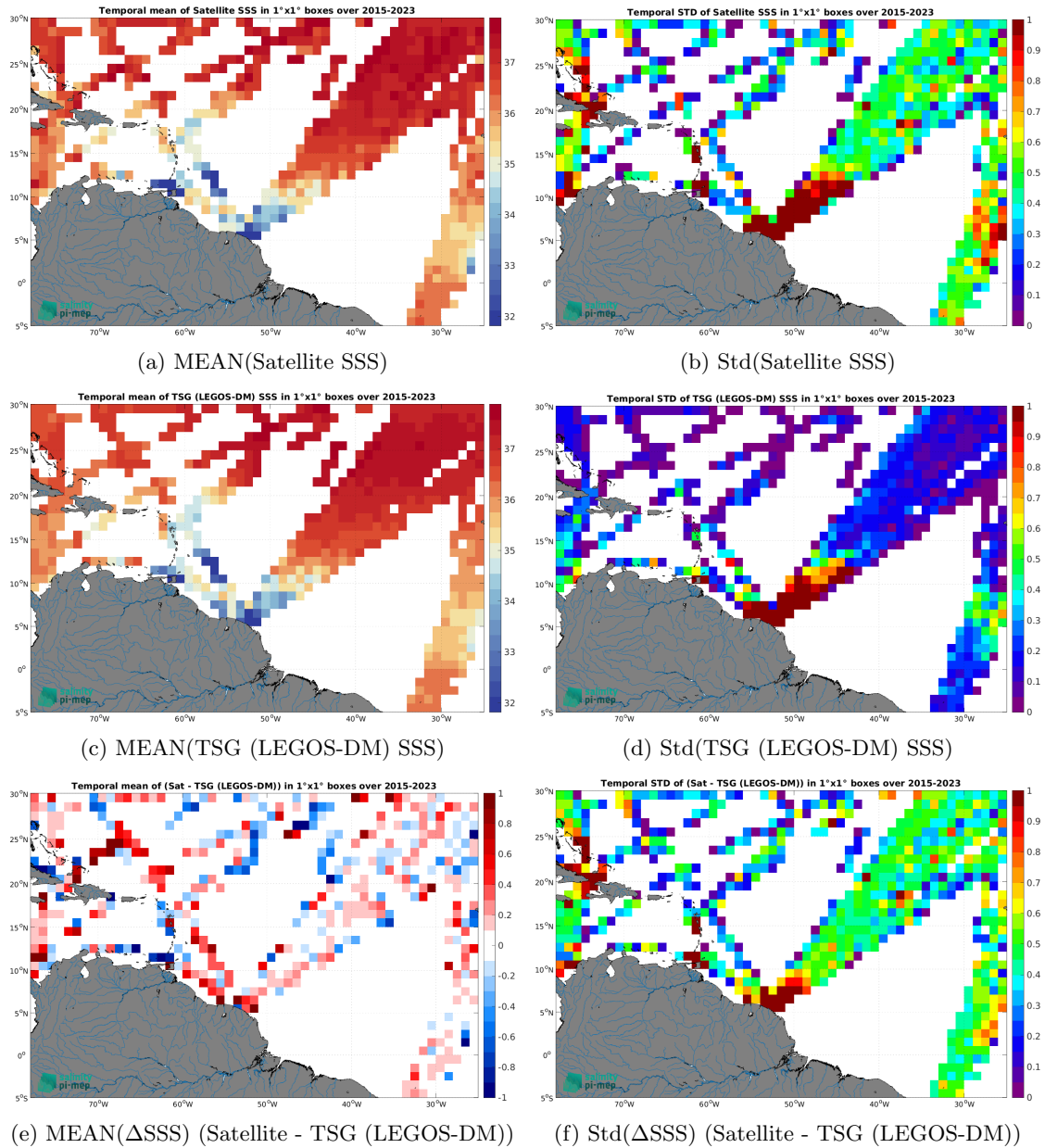
Figure 7: Temporal mean (left) and Std (right) of SSS from SMAP SSS L2 v5.0 (JPL) (top), TSG (LEGOS-DM) (middle), and of \Delta SSS (Satellite - TSG (LEGOS-DM)). Only match-up pairs are used to generate these maps.
