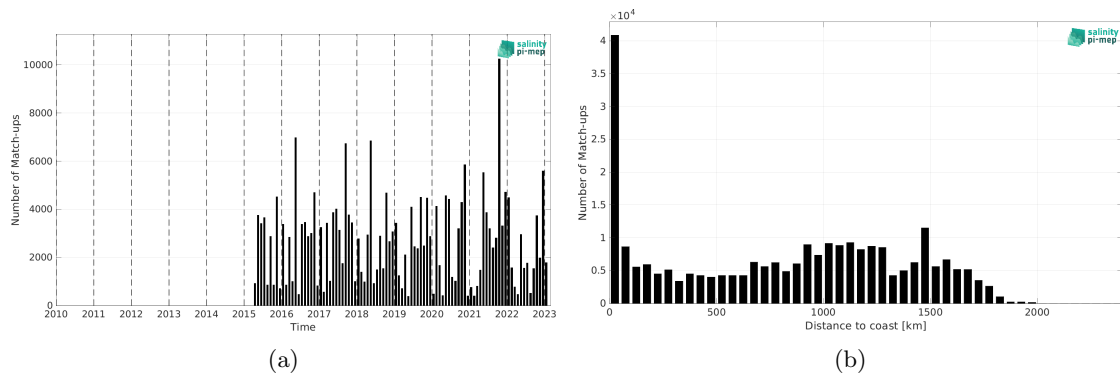
Figure 2: Number of match-ups between TSG (LEGOS-DM) and SMAP SSS L2 v5.0 (JPL) SSS as a function of time (a) and as function of the distance to coast (b) over the Amazon and Orinoco river plumes Pi-MEP region and for the full satellite product period.
