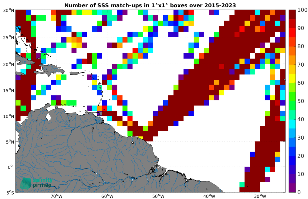
Figure 5: Number of SSS match-ups between TSG (LEGOS-DM) SSS and the SMAP SSS L2 v5.0 (JPL) SSS product for the Amazon and Orinoco river plumes Pi-MEP region over 1^\circ \times 1^\circ boxes and for the full satellite product period.
