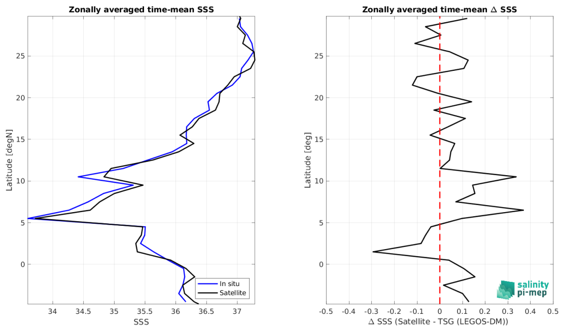
Figure 9: Left panel: Zonal mean SSS from SMAP SSS L2 v5.0 (JPL) satellite product (black) and from TSG (LEGOS-DM) (blue). Right panel: Zonal mean of \Delta SSS (Satellite - TSG (LEGOS-DM)) for all the collected Pi-MEP match-up pairs estimated over the full satellite product period.
