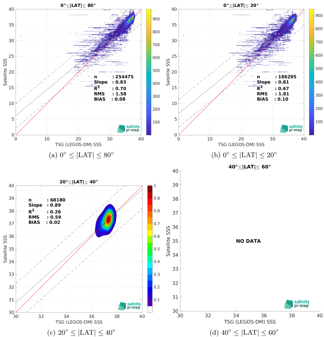
Figure 10: Contour maps of the concentration of SMAP SSS L2 v5.0 (JPL) SSS (y-axis) versus TSG (LEGOS-DM) SSS (x-axis) at match-up pairs for different latitude bands. For each plot, the red line shows x=y . The black thin and dashed lines indicate a linear fit through the data cloud and the \pm 95\% confidence levels, respectively. The number match-up pairs n , the slope and R^2 coefficient of the linear fit, the root mean square (RMS) and the mean bias between satellite and in situ data are indicated for each latitude band in each plots.
