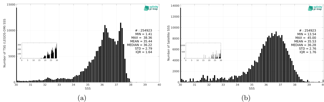
Figure 3: Histograms of SSS from TSG (LEGOS-DM) (a) and SMAP SSS L2 v5.0 (JPL) (b) considering all match-up pairs per bins of 0.1 over the Amazon and Orinoco river plumes Pi-MEP region and for the full satellite product period.
