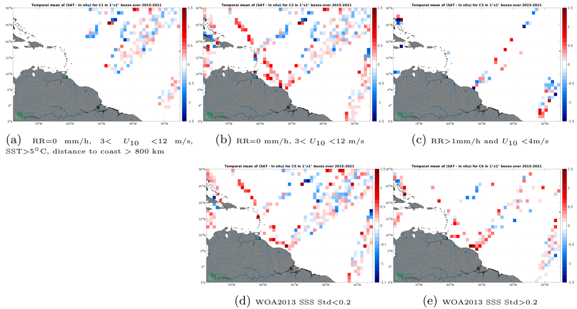
Figure 12: Temporal mean gridded over spatial boxes of size 1^\circ \times 1^\circ of \Delta SSS (SMAP SSS L2 v5.0 (JPL) - TSG (LEGOS-DM)) for 5 different subdatasets corresponding to: RR=0 mm/h, 3 < U_{10} < 12 m/s, SST > 5^\circ\text{C} , distance to coast > 800 km (a), RR=0 mm/h, 3 < U_{10} < 12 m/s (b), RR > 1 mm/h and U_{10} < 4 m/s (c), WOA2013 SSS Std < 0.2 (d), WOA2013 SSS Std > 0.2 (e).
