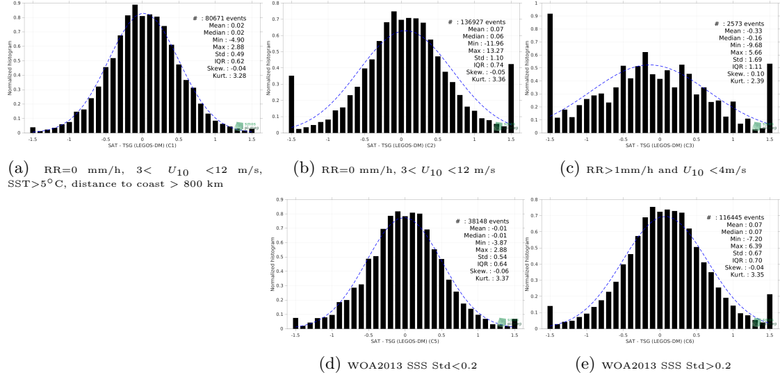
Figure 13: Normalized histogram of \Delta SSS (SMAP SSS L2 v5.0 (JPL) - TSG (LEGOS-DM)) for 5 different subdatasets corresponding to: RR=0 mm/h, 3 < U_{10} < 12 m/s, SST >5^{\circ} C, distance to coast > 800 km (a), RR=0 mm/h, 3 < U_{10} < 12 m/s (b), RR >1 mm/h and U_{10} < 4 m/s (c), WOA2013 SSS Std <0.2 (d), WOA2013 SSS Std >0.2 (e).
