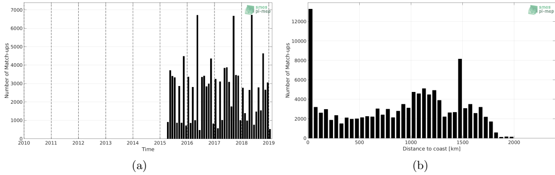
Figure 1: Number of match-ups between TSG (LEGOS-DM) and SMAP SSS L2 v5.0 (JPL) SSS as a function of time (a) and as function of the distance to coast (b) over the Amazon and Orinoco river plumes Pi-MEP region and for the full satellite product period.
