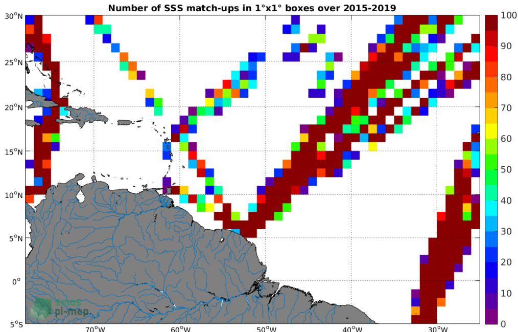
Figure 4: Number of SSS match-ups between TSG (LEGOS-DM) SSS and the SMAP SSS L2 v5.0 (JPL) SSS product for the Amazon and Orinoco river plumes Pi-MEP region over 1°x1° boxes and for the full satellite product period.
