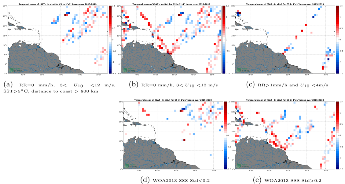
Figure 12: Temporal mean gridded over spatial boxes of size 1°x1° of \Delta SSS (SMAP SSS L2 v5.0 (JPL) - TSG (LEGOS-DM)) for 5 different subdatasets corresponding to: RR=0 mm/h, 3 < U_{10} < 12 m/s, SST > 5°C, distance to coast > 800 km (a), RR=0 mm/h, 3 < U_{10} < 12 m/s (b), RR > 1mm/h and U_{10} < 4 m/s (c), WOA2013 SSS Std < 0.2 (d), WOA2013 SSS Std > 0.2 (e).
