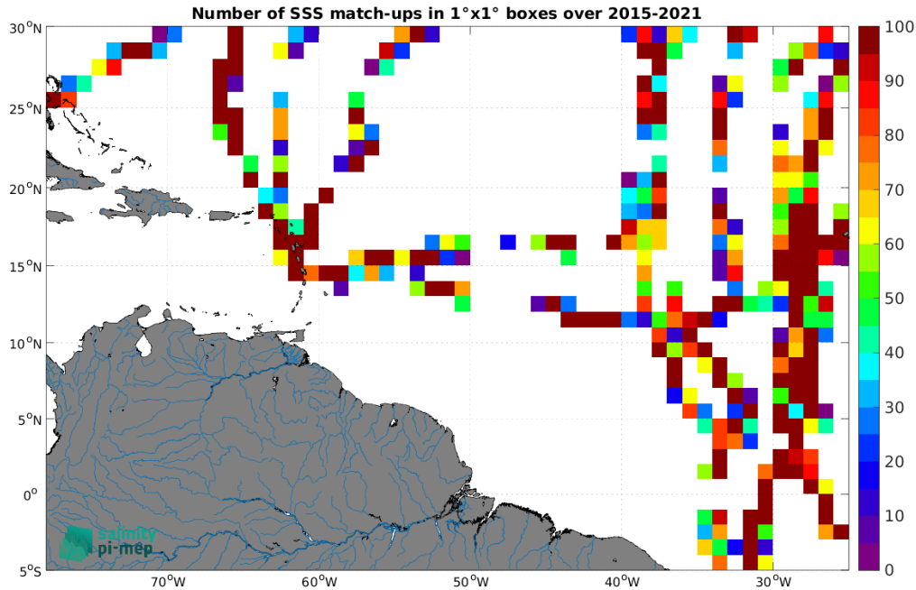
Figure 5: Number of SSS match-ups between TSG (GOSUD-Sailing-ship) SSS and the SMAP SSS L2 v5.0 (JPL) SSS product for the Amazon and Orinoco river plumes Pi-MEP region over 1^\circ \times 1^\circ boxes and for the full satellite product period.
