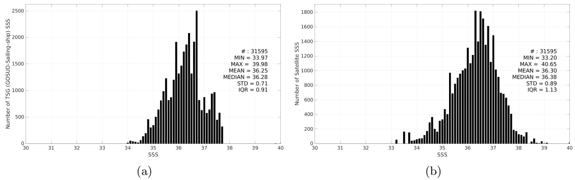
Figure 3: Histograms of SSS from TSG (GOSUD-Sailing-ship) (a) and SMAP SSS L2 v5.0 (JPL) (b) considering all match-up pairs per bins of 0.1 over the Amazon and Orinoco river plumes Pi-MEP region and for the full satellite product period.
