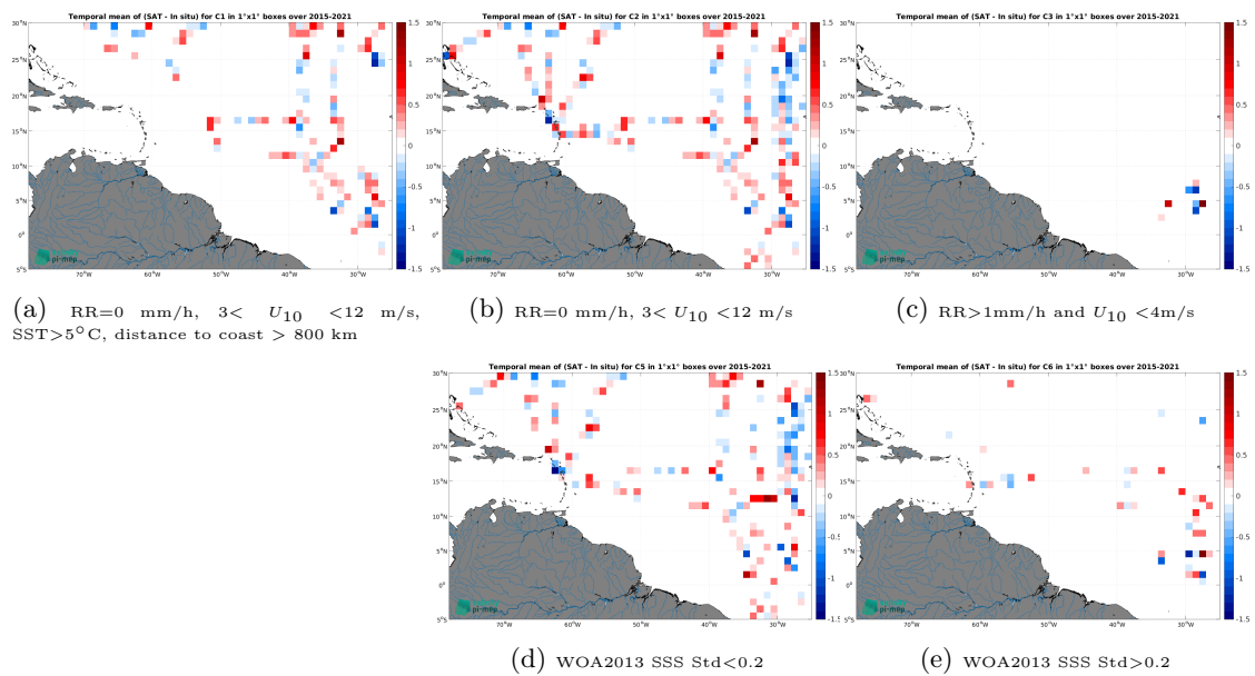
Figure 14: Temporal mean gridded over spatial boxes of size 1^\circ \times 1^\circ of \Delta\text{SSS} (SMAP SSS L2 v5.0 (JPL) - TSG (GOSUD-Sailing-ship)) for 5 different subdatasets corresponding to:RR=0 mm/h, 3 < U_{10} < 12 m/s, SST >5^\circ\text{C} , distance to coast > 800 km (a), RR=0 mm/h, 3 < U_{10} < 12 m/s (b), RR >1 mm/h and U_{10} < 4 m/s (c), WOA2013 SSS Std <0.2 (d), WOA2013 SSS Std >0.2 (e).
