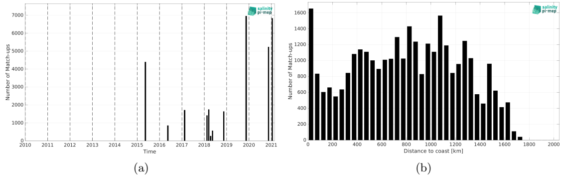
Figure 2: Number of match-ups between TSG (GOSUD-Sailing-ship) and SMAP SSS L2 v5.0 (JPL) SSS as a function of time (a) and as function of the distance to coast (b) over the Amazon and Orinoco river plumes Pi-MEP region and for the full satellite product period.
