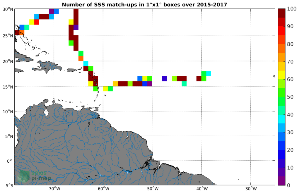
Figure 4: Number of SSS match-ups between TSG (GOSUD-Sailing-ship) SSS and the SMAP SSS L2 v5.0 (JPL) SSS product for the Amazon and Orinoco river plumes Pi-MEP region over 1°x1° boxes and for the full satellite product period.
