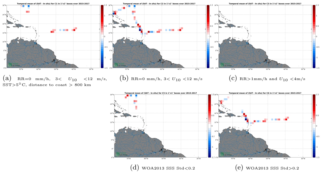
Figure 12: Temporal mean gridded over spatial boxes of size 1°x1° of \Delta SSS (SMAP SSS L2 v5.0 (JPL) - TSG (GOSUD-Sailing-ship)) for 5 different subdatasets corresponding to: RR=0 mm/h, 3 < U_{10} < 12 m/s, SST > 5°C, distance to coast > 800 km (a), RR=0 mm/h, 3 < U_{10} < 12 m/s (b), RR > 1mm/h and U_{10} < 4 m/s (c), WOA2013 SSS Std < 0.2 (d), WOA2013 SSS Std > 0.2 (e).
