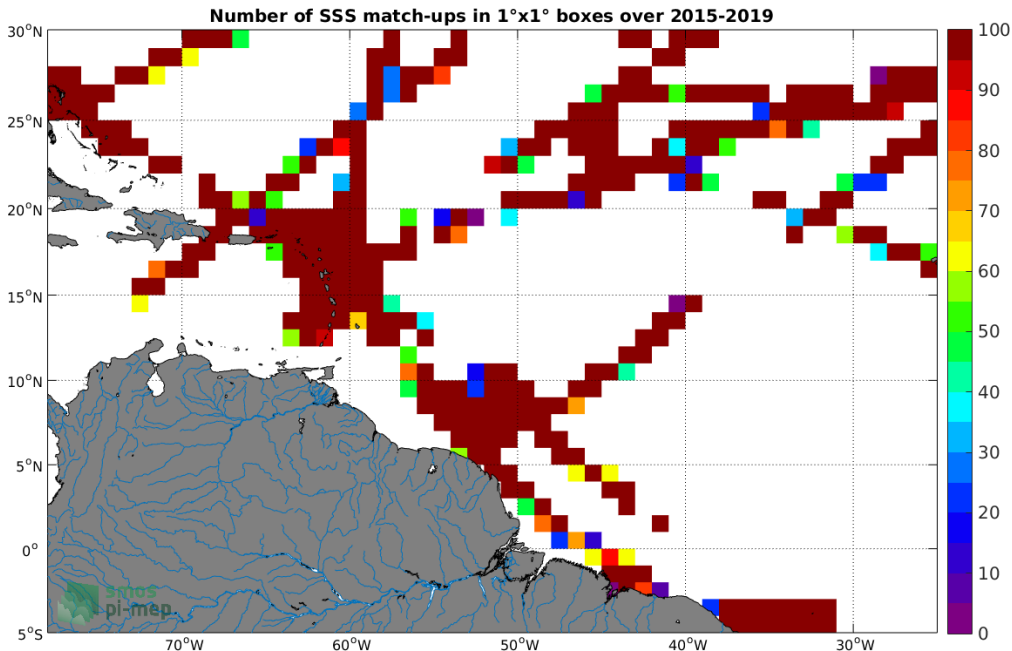
Figure 4: Number of SSS match-ups between TSG (GOSUD-Research-vessel) SSS and the SMAP SSS L2 v5.0 (JPL) SSS product for the Amazon and Orinoco river plumes Pi-MEP region over 1°x1° boxes and for the full satellite product period.
