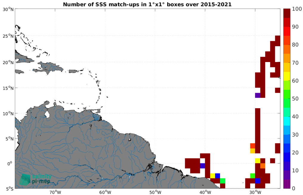
Figure 5: Number of SSS match-ups between TSG (CSIC-UTM) SSS and the SMAP SSS L2 v5.0 (JPL) SSS product for the Amazon and Orinoco river plumes Pi-MEP region over 1^\circ \times 1^\circ boxes and for the full satellite product period.
